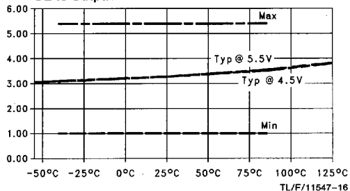
t_{PLZ} vs Temperature ( T_A ) C_L = 50\text{ pF} , 1 Output Switching \overline{OE} to Output
