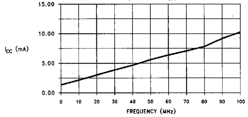
Typical I CC vs Output Switching Frequency C L = 0 pF, V CC = V IH = 5.5V, LE = GND, 1 Output Switching at 50% Duty Cycle Data to Output, Transparent Mode with Unused Data Inputs = V IH
