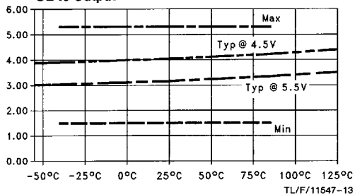
t_{PZH} vs Temperature ( T_A ) C_L = 50\text{ pF} , 1 Output Switching \overline{OE} to Output
