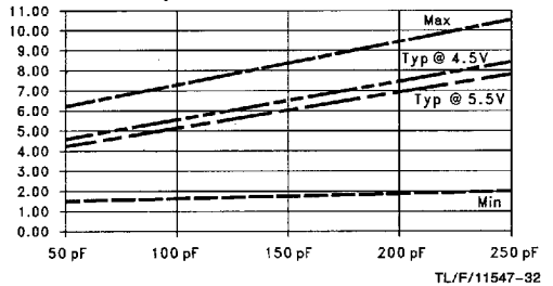
tpZL vs Load Capacitance TA = 25°C, 8 Outputs Switching OE to Output
