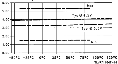
t_{PZL} vs Temperature ( T_A ) C_L = 50\text{ pF} , 1 Output Switching \overline{OE} to Output
