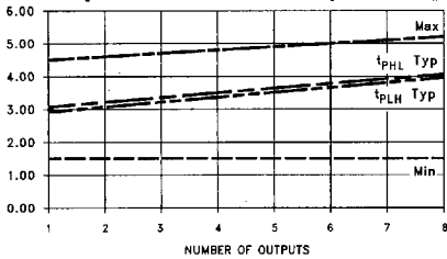
t PLH and t PHL vs Number Outputs Switching C L = 50 pF, T A = 25°C, V CC = 5.0V, Outputs In Phase Data to Output
