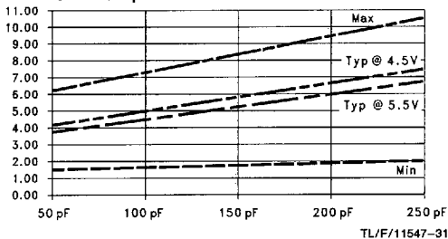
tpZH vs Load Capacitance TA = 25°C, 8 Outputs Switching OE to Output
