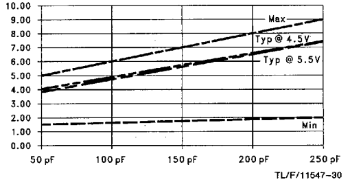
tpHL vs Load Capacitance TA = 25°C, 8 Outputs Switching Data to Output
