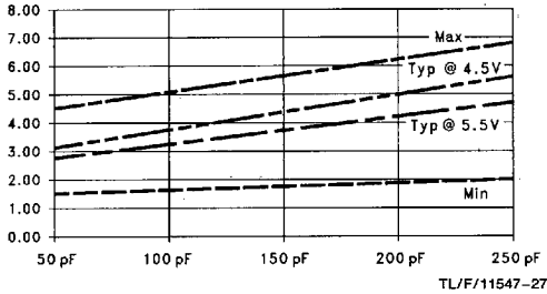
tpLH vs Load Capacitance TA = 25°C, 1 Output Switching Data to Output
