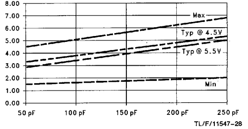
tpHL vs Load Capacitance TA = 25°C, 1 Output Switching Data to Output
