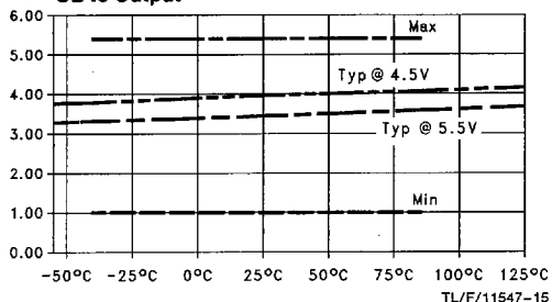
t_{PHZ} vs Temperature ( T_A ) C_L = 50\text{ pF} , 1 Output Switching \overline{OE} to Output
