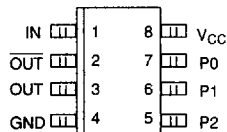
DS1040Z 8-PIN SOIC (150 MIL) See Mech. Drawing – Pg. 483
