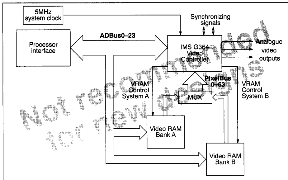
Figure 14.3 IMS G364 operating with an interleaved memory system
