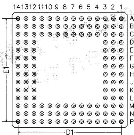
Figure 14.5 132 pin grid array package dimensions
