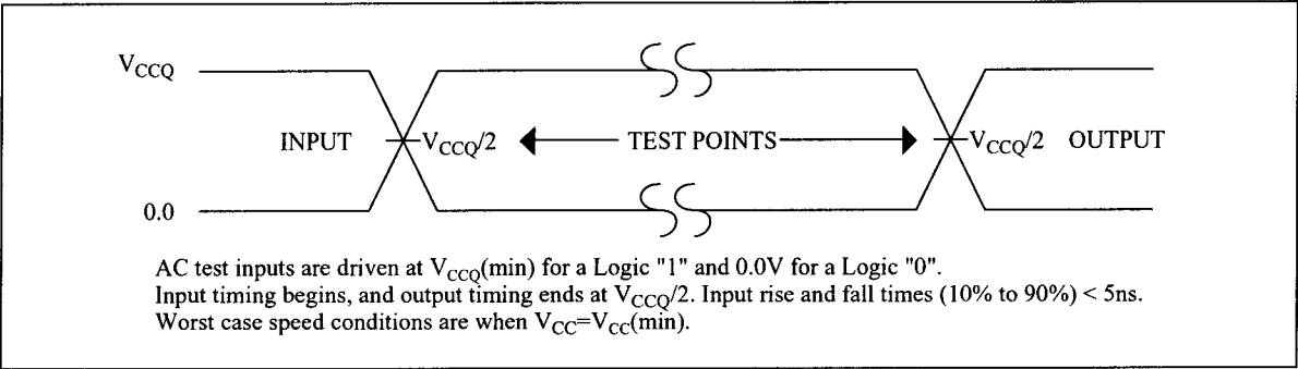
Figure 5. Transient Input/Output Reference Waveform for V_{\text{CC}}=2.7\text{V}-3.6\text{V}
