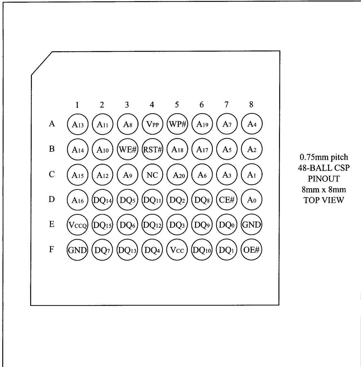
Figure 1. 0.75mm pitch 48-Ball CSP (8mm×8mm) Pinout
