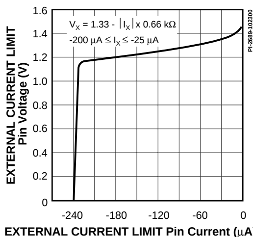
Figure 62b. EXTERNAL CURRENT LIMIT Pin Voltage vs. Current.
