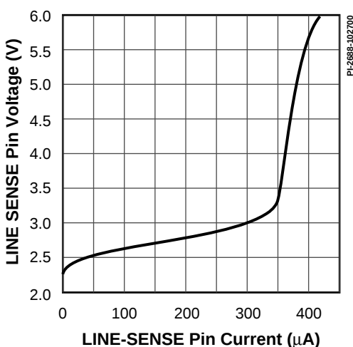
Figure 62a. LINE-SENSE Pin Voltage vs. Current.
