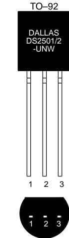
BOTTOM VIEW See Mech. Drawings Section
