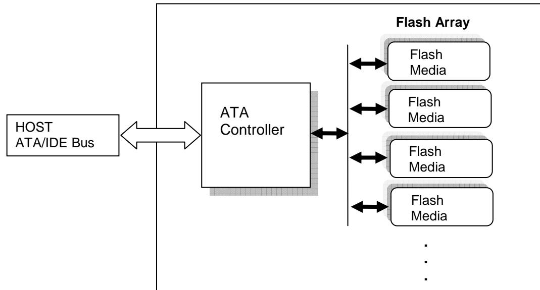
Figure 2-1: ATA-Flash Drive functional block diagram
