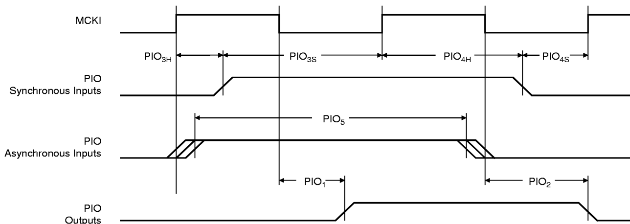
Figure 11. PIO Signals Relative to MCKI
