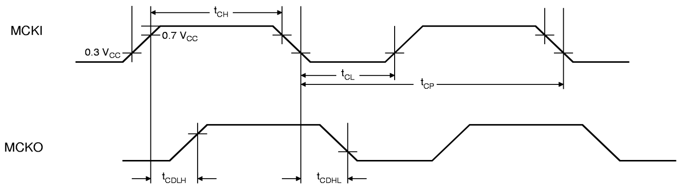
Figure 12. Clock Waveform
