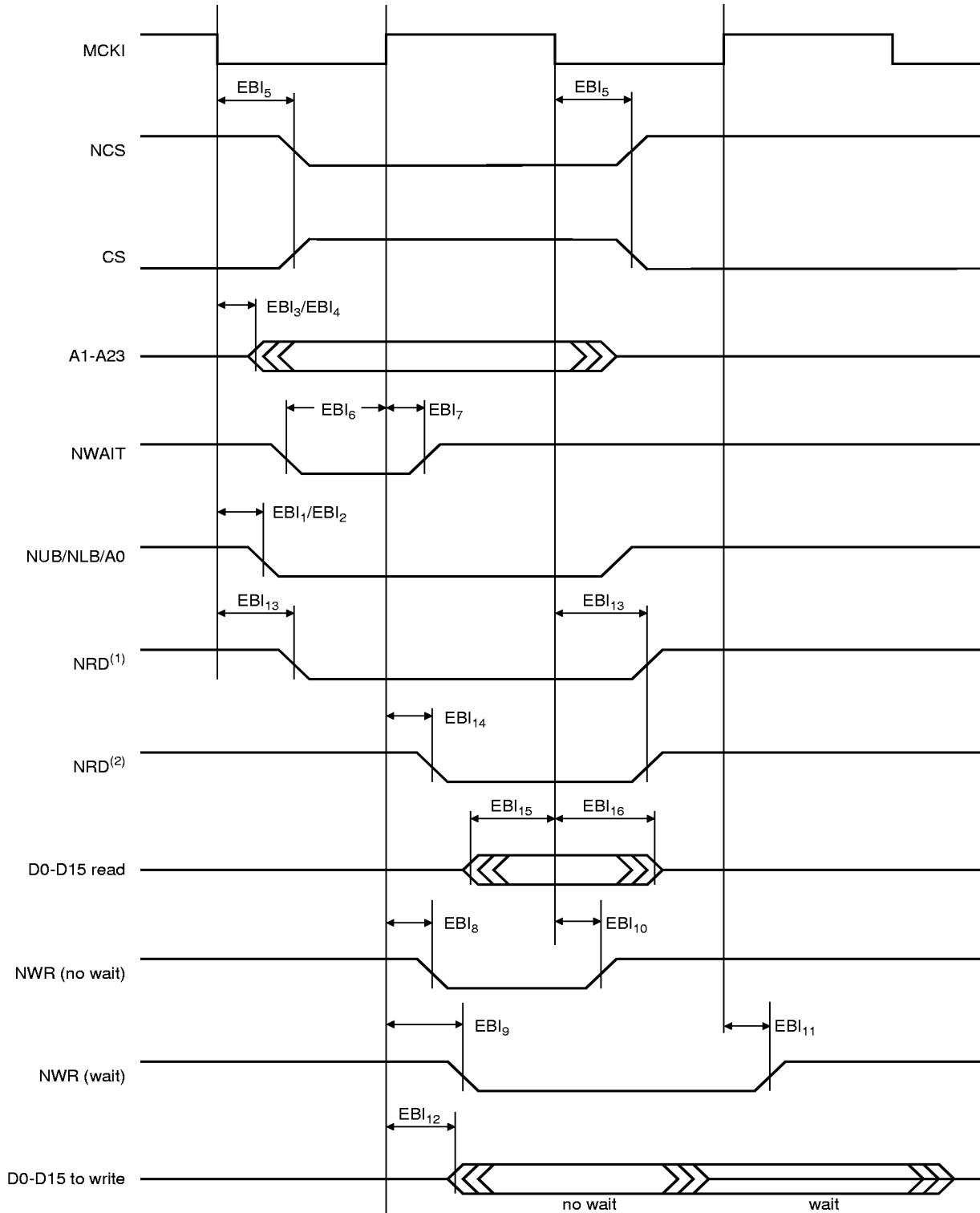
Figure 5. EBI Signals Relative to MCKI
