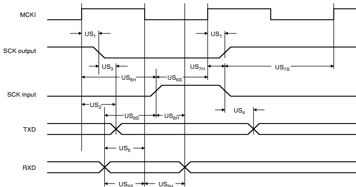
Figure 6. USART Signals Relative to MCKI
