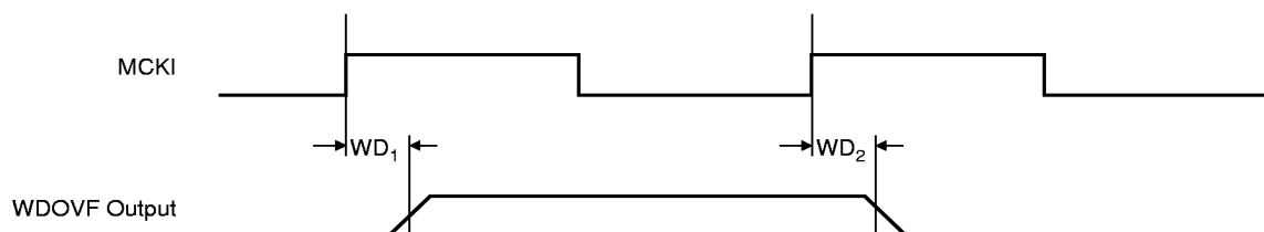
Figure 8. Watchdog Signals Relative to MCKI
