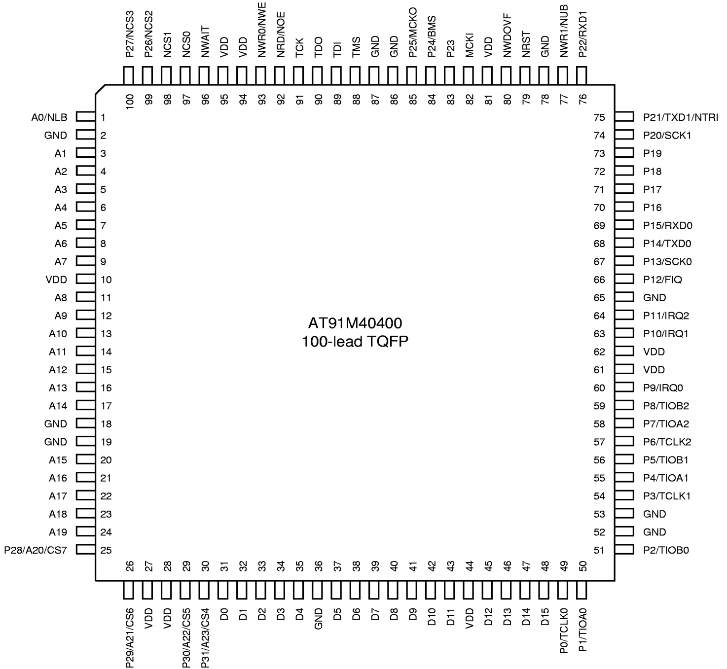
Figure 1. AT91M40400 Pinout (Top View)
