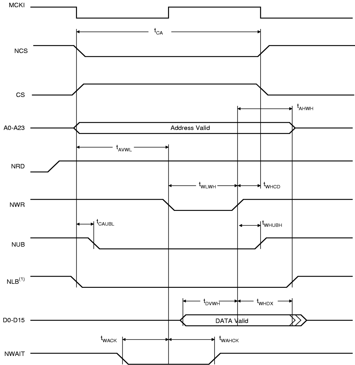
Figure 4. External Data Memory Write Cycle
