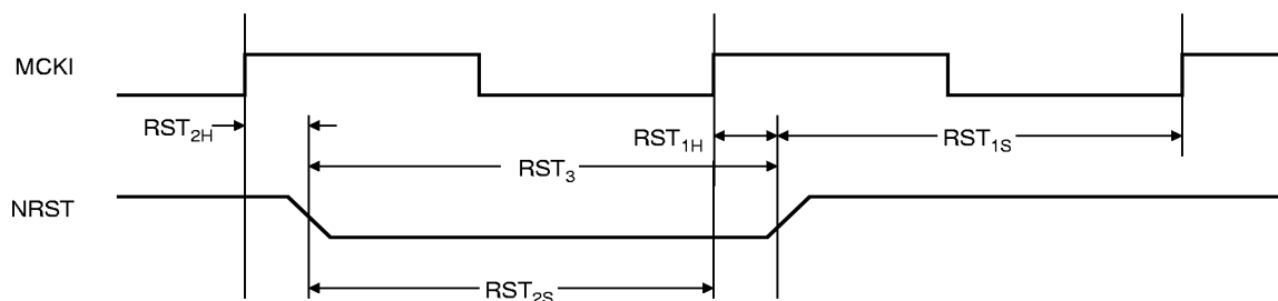
Figure 9. Reset Signals Relative to MCKI
