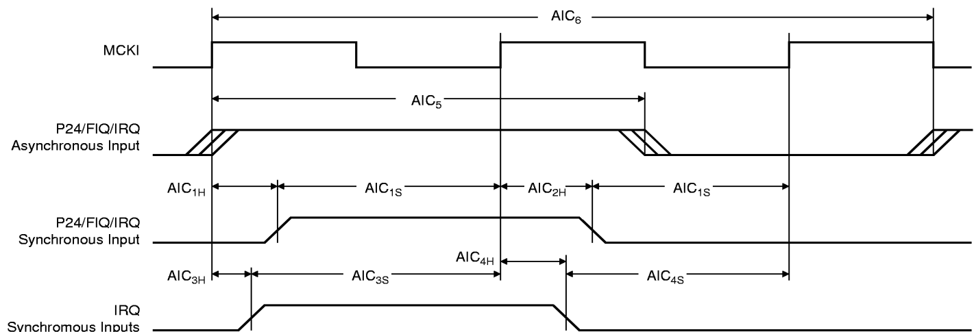
Figure 10. AIC Signals Relative to MCKI
