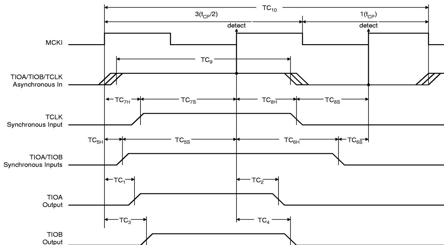
Figure 7. Timer Relative to MCKI
