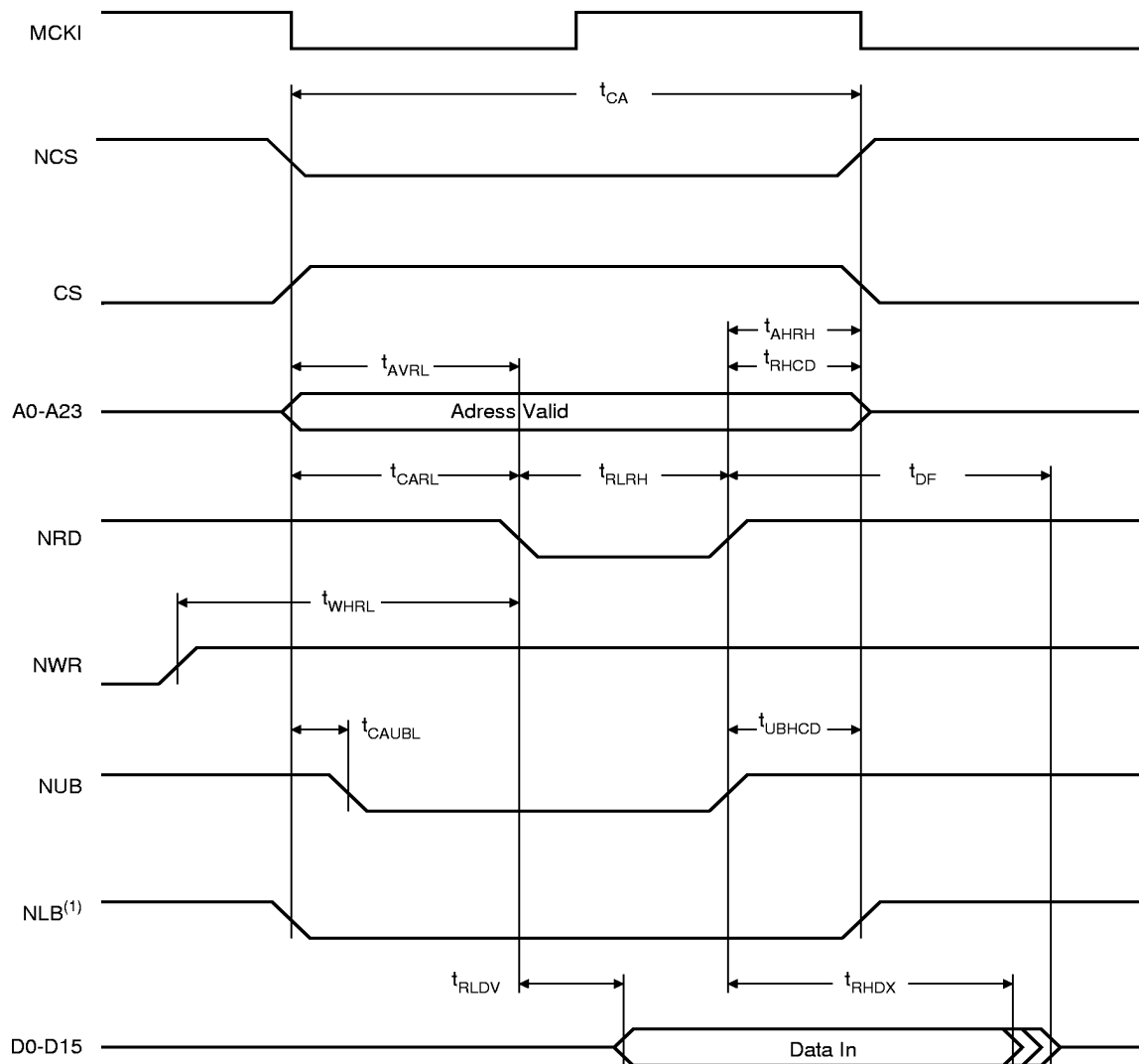
Figure 3. External Data Memory Read Cycle
