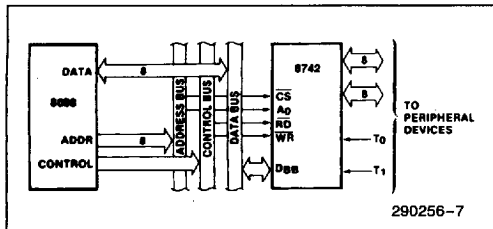
Figure 3. 8088-8742 Interface
