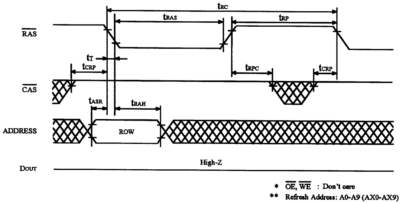
FIGURE 5. \overline{RAS} ONLY REFRESH CYCLE
