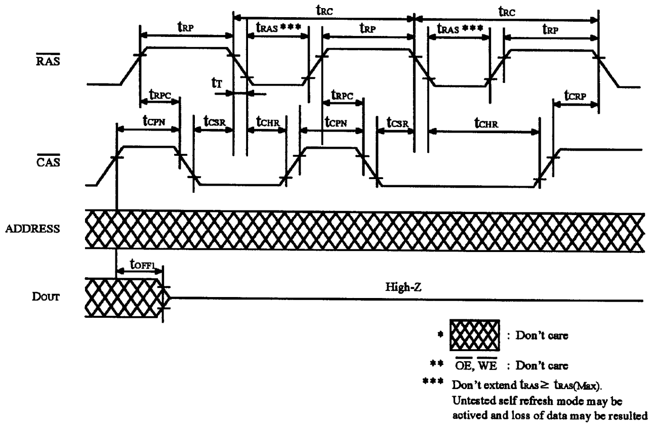
FIGURE 6. \overline{CAS} BEFORE \overline{RAS} REFRESH CYCLE
