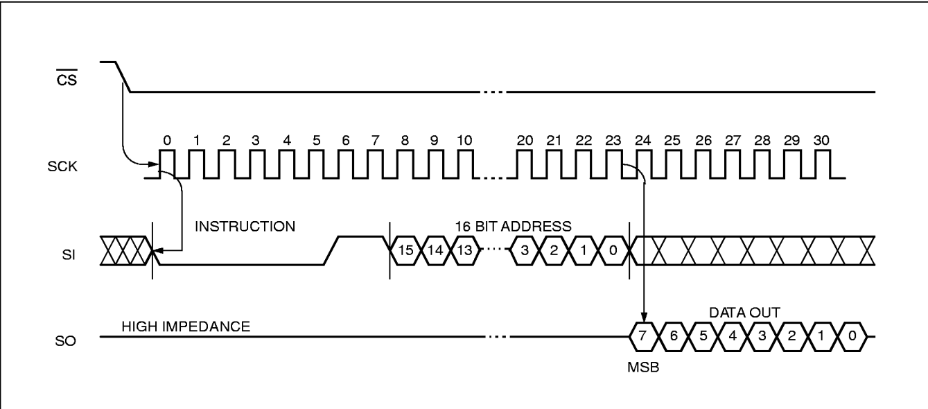
Figure 5. Read EEPROM Array Sequence
