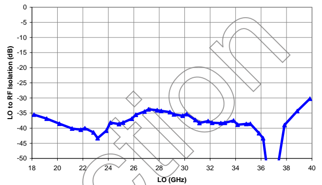
XM1004-BD: LO to RF Isolation (dB) vs LO Freq (GHz) LO = +12 dBm, Vg = -0.5 V
