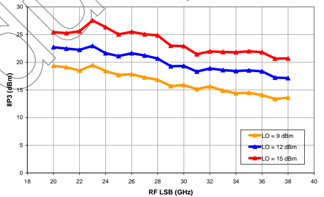
XM1004-BD: IIP3 (dBm) vs. RF LSB (GHz) IF = 2 GHz at -13 dBm per Tone
