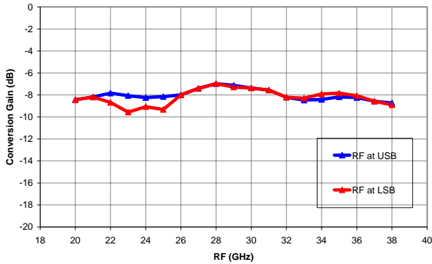
XM1004-BD: Conversion Gain (dB) vs RF Freq (GHz) IF = 1.8 GHz, IF Pin = -10 dBm, LO = +12 dBm
