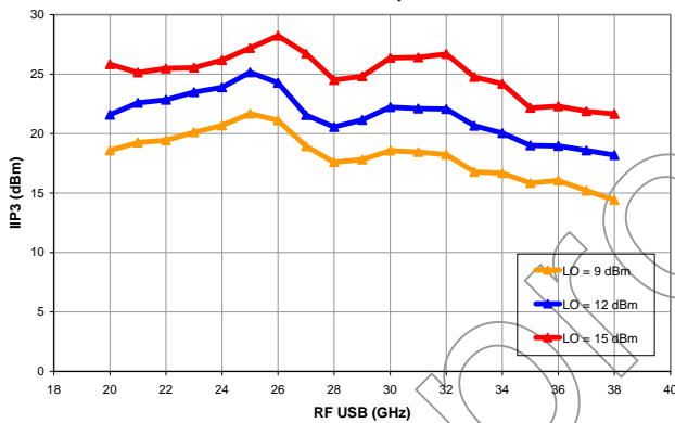
XM1004-BD: IIP3 (dBm) vs. RF USB (GHz) IF = 2 GHz at -13 dBm per Tone
