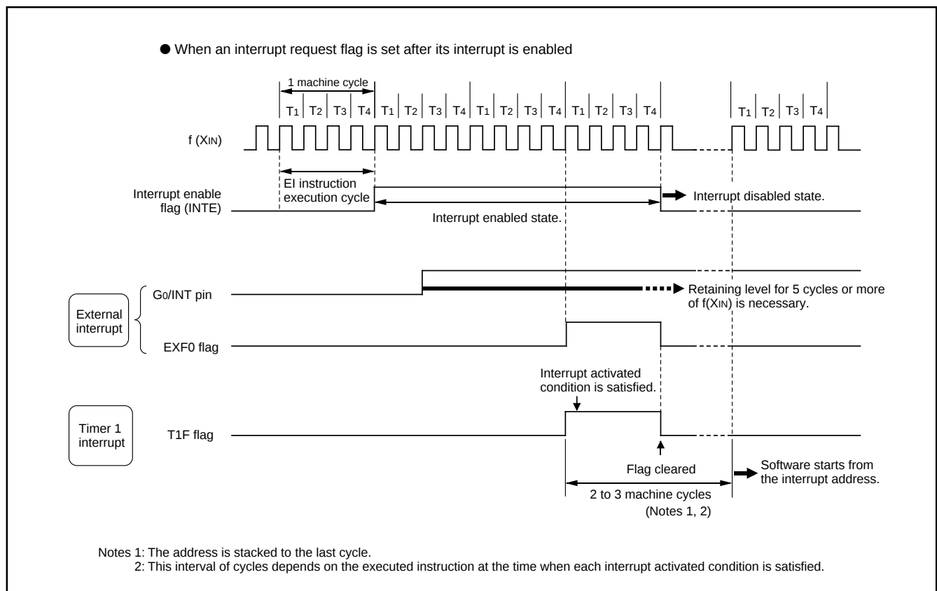
Fig. 16 Interrupt sequence
