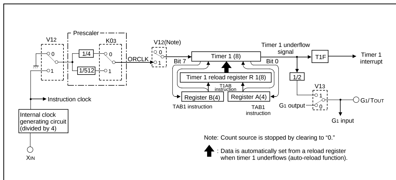
Fig. 19 Timers structure
