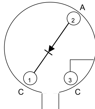
TO-72 (Bottom View)
