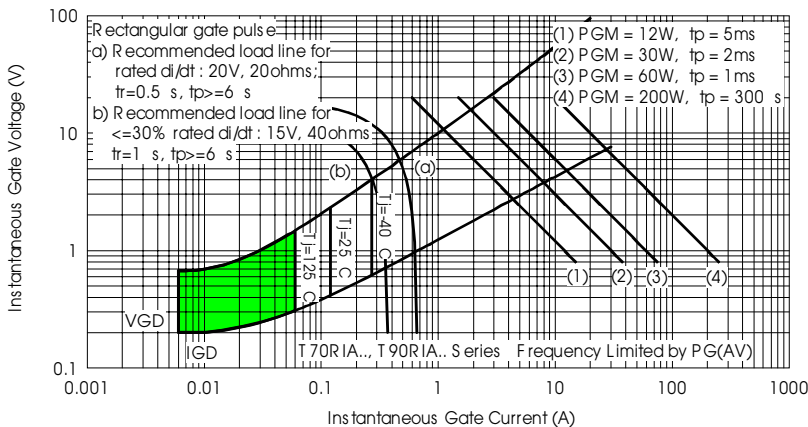
Fig. 19 - Gate Characteristics
