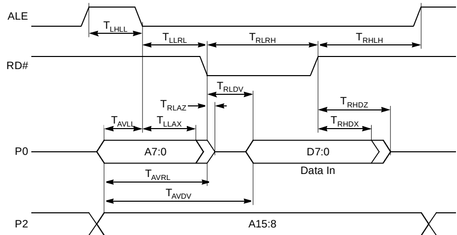
Figure 16. External 8-bit Bus Cycle – Data Read Waveforms
