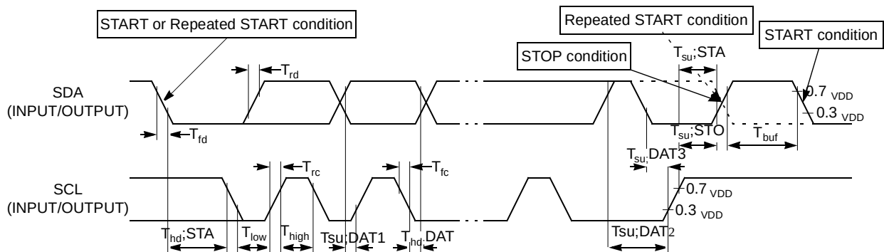
Figure 24. Two-wire Waveforms
