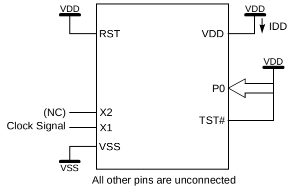
I_{DD} , I_{DL} and I_{PD} Test Conditions Figure 10. I_{DD} Test Condition, Active Mode
