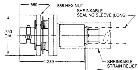
INSULATED BULKHEAD JACK REAR MOUNT, TOOL CRIMP
