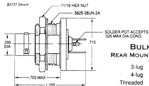
FEED-THROUGH JACK
