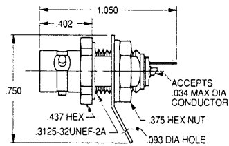
BULKHEAD JACK FRONT MOUNT, SOLDER POT
