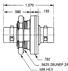
INSULATED FEED-THROUGH JACK
