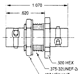
FEED-THROUGH JACK
