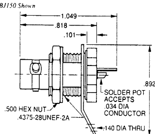
BULKHEAD JACK REAR MOUNT, SOLDER POT
