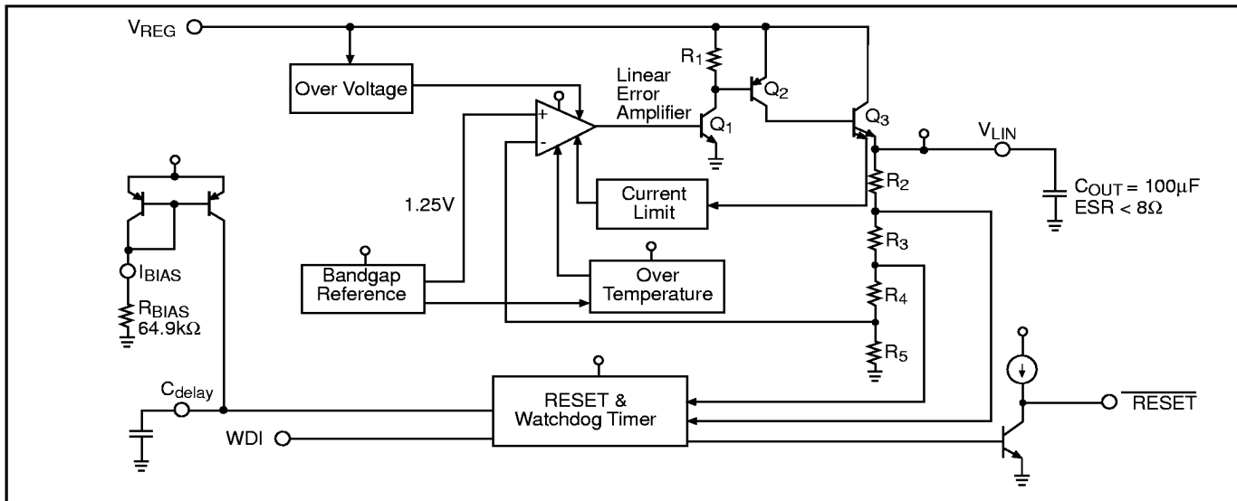
Figure 2. Block diagram of 5V linear regulator portion of the CS-5111.
