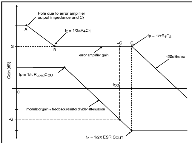
Figure 10. Bode plot of error amplifier (OTA) gain and modulator gain added to the feedback resistor divider attenuation.
