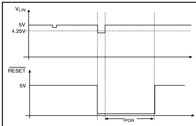
Figure 5b. \overline{\text{RESET}} signal is issued whenever V_{\text{LIN}} falls below 4.25V (typical).
