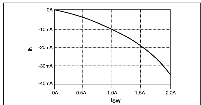
Figure 1b. Supply Current vs. Switch Current.
