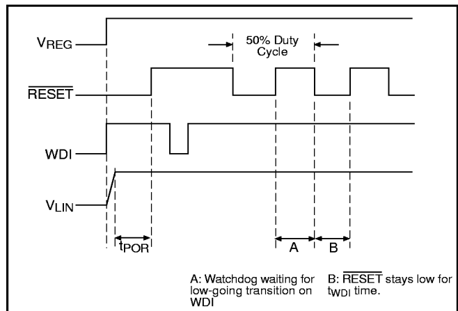
Figure 4. Timing diagram when WDI fails to appear within the preset time interval, t_{WDI} .
