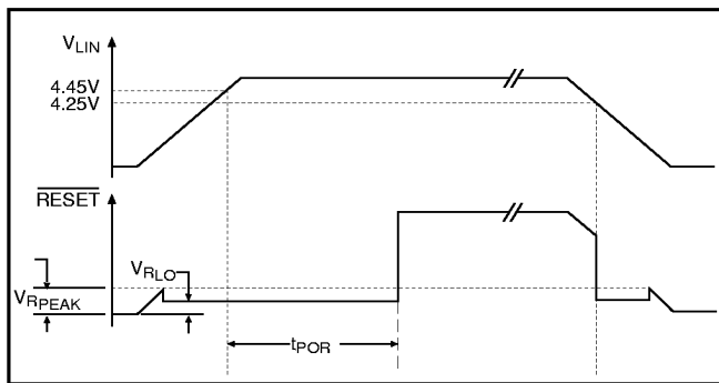
Figure 5a. The power on reset time interval ( t_{\text{POR}} ) begins when V_{\text{LIN}} rises above 4.45V (typical).
