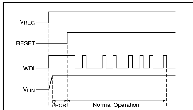
Figure 3. Timing diagram for normal regulator operation.
