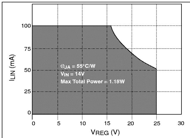
Figure 12: The shaded area shows the safe operating area of the CS-5111 as a function of I_{\text{LIN}} , V_{\text{REG}} , and \Theta_{\text{JA}} . Refer to the table below for typical loads and voltages.
