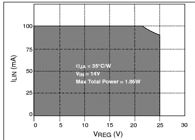
Figure 12: The shaded area shows the safe operating area of the CS-5111 as a function of I_{\text{LIN}} , V_{\text{REG}} , and \Theta_{\text{JA}} . Refer to the table below for typical loads and voltages.
