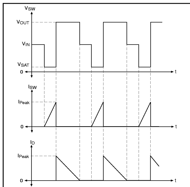
Figure 7: Voltage and current waveforms for boost topology in CS-5111.
