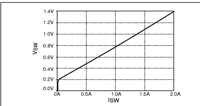
Figure 1c. Switch Saturation Voltage.
