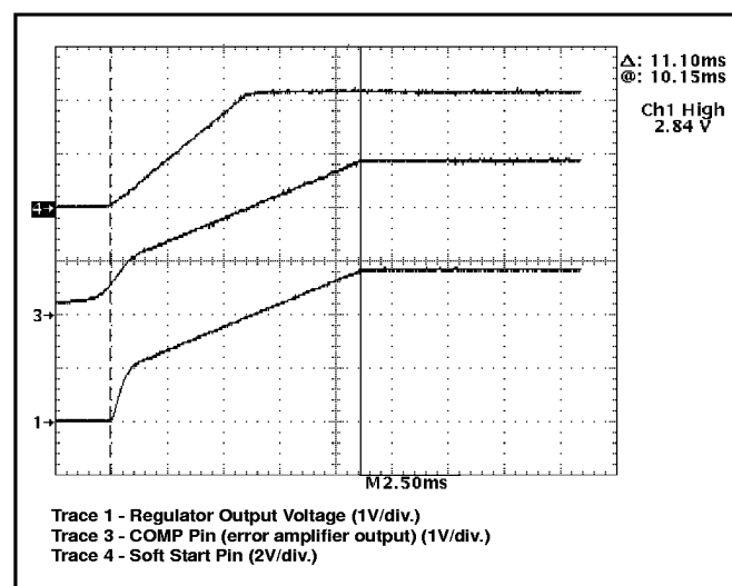
Figure 3: CS-5150H demonstration board startup waveforms.
