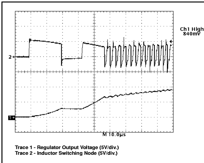
Figure 4: CS-5150H demonstration board enable startup waveforms.
