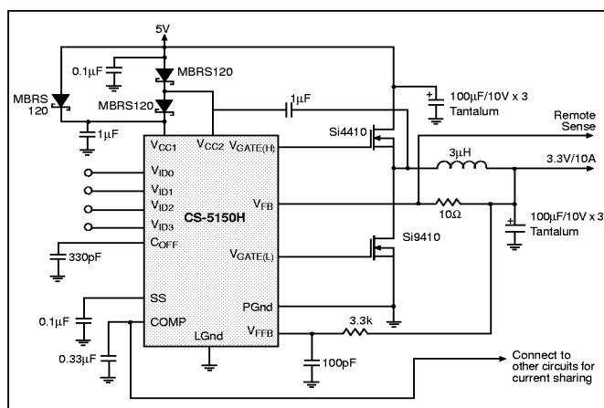
Figure 22: 5V to 3.3V/10A converter with current sharing.
