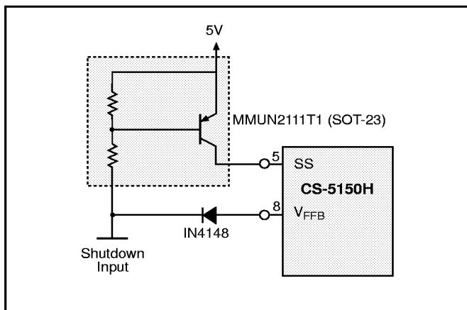
Figure 14: Implementing shutdown with the CS-5150H.
