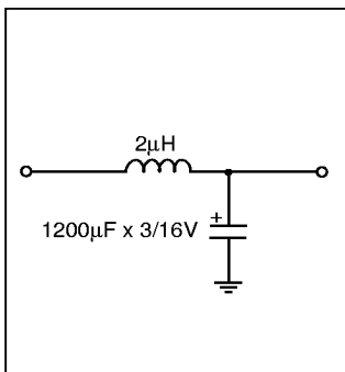
Figure 19: Input Filter
