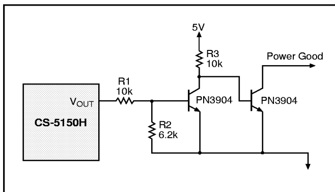
Figure 15: Implementing Power Good with the CS-5150H.
