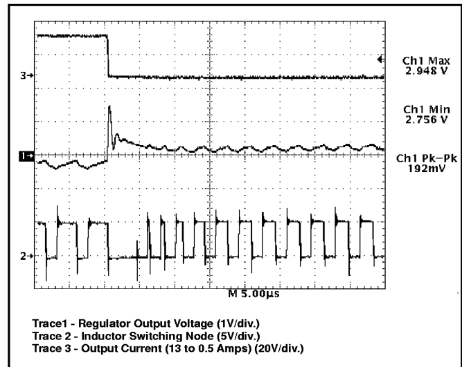
Figure 9: CS-5150H demonstration board response to 13A load turn off (output set for 2.8V). V^{2TM} control topology immediately connects inductor to ground, providing 0% duty cycle. Regulation is achieved in less than 10µs.
