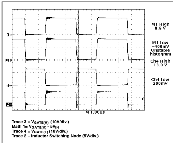
Figure 17: CS-5150H gate drive waveforms depicting rail to rail swing.
