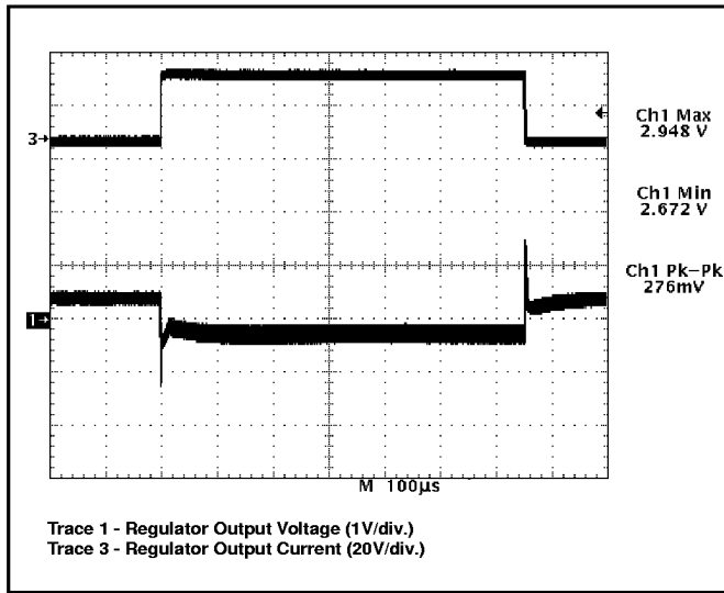
Figure 7: CS-5150H demonstration board response to a 0.5 to 13A load pulse (output set for 2.8V).
