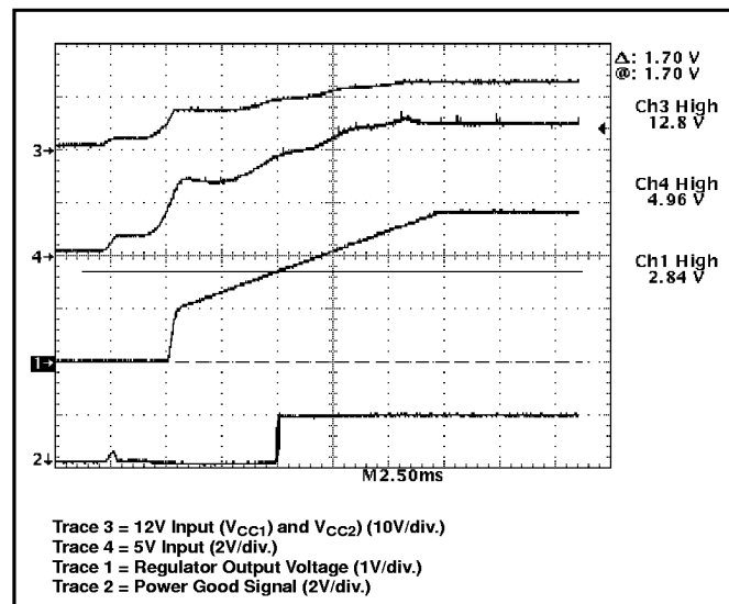
Figure 16: CS-5150H demonstration board during power up. Power Good signal is activated when output voltage reaches 1.70V.
