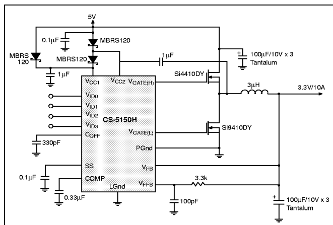
Figure 21: 5V to 3.3V/10A converter.
