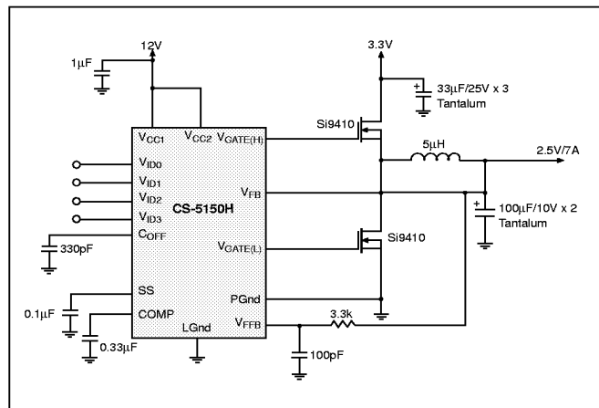
Figure 24: 3.3V to 2.5V/7A converter with 12V bias.
