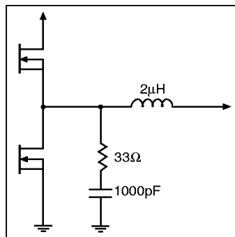
Figure 18: Filter components
