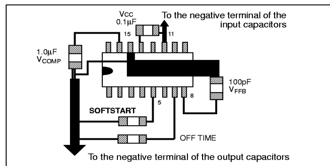
Figure 20: Layout Guidelines
