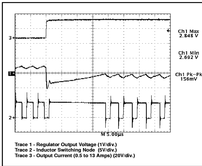
Figure 8: CS-5150H demonstration board response to 13A load turn on (output set for 2.8V). Upon completing a normal off time, the V^{2TM} control loop immediately connects the inductor to the input voltage, providing 100% duty cycle. Regulation is achieved in less than 20µs.
