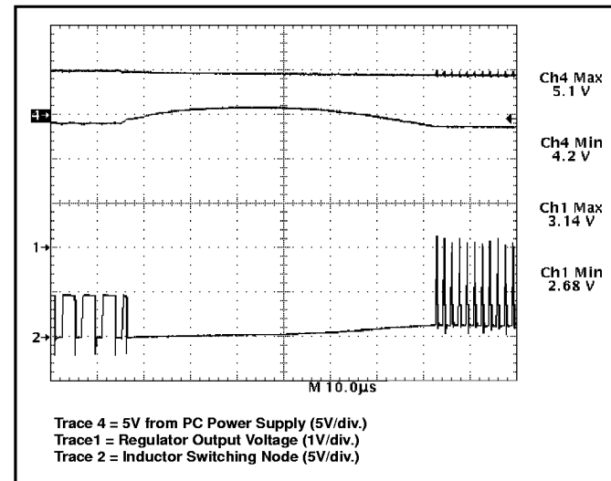
Figure 12: OVP response to an input-to-output short circuit by immediately providing 0% duty cycle, crow-barring the input voltage to ground.
