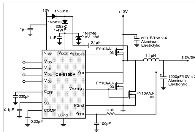
Figure 23: 12V to 3.3V/5A converter with remote sense.
