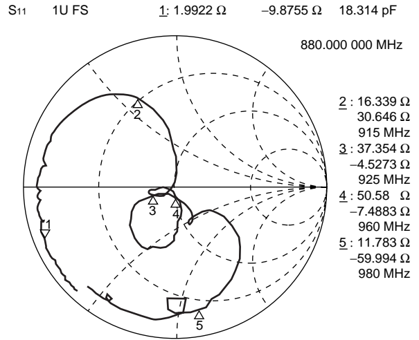
CENTER 950 MHz SPAN 300 MHz
