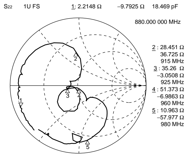
CENTER 950 MHz SPAN 300 MHz
