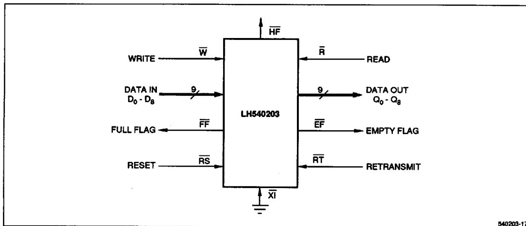
Figure 4. Standalone FIFO (2048 × 9)
