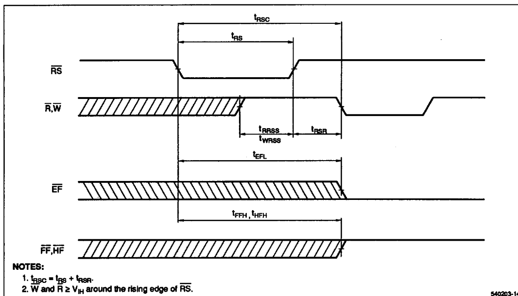
Figure 10. Reset Timing
