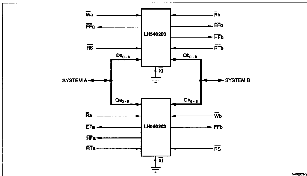
Figure 8. Bidirectional FIFO Operation (2048 \times 9 \times 2)
