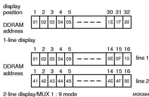
Fig.4 DDRAM to display mapping; left shift: (For 1 \times 32 only as long as 4F and 00 positions are not on display simultaneously).
