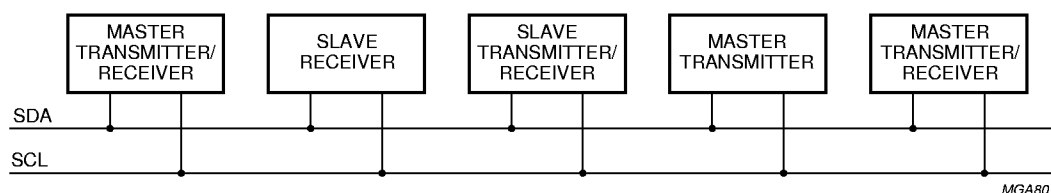
Fig.18 System configuration.
