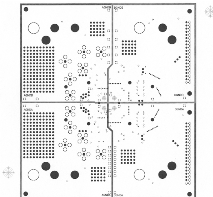
Figure 11c. GND1
