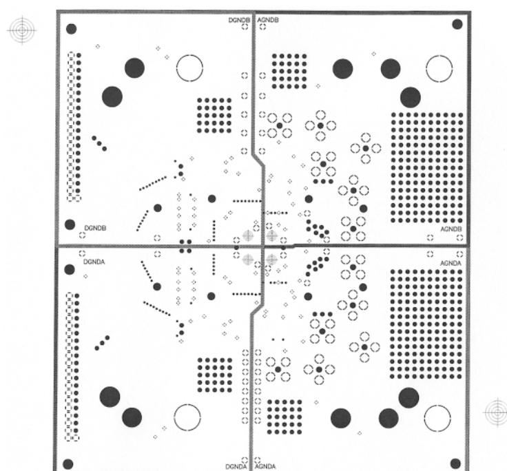
Figure 11d. GND2
