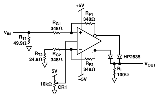
Figure 19. Full-Wave Rectifier
