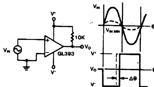
Figure 9-Time Delay Generator
