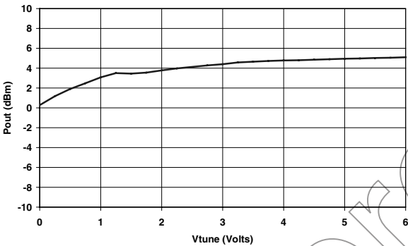
XQ1000-BD Output Power vs. Tuning Voltage
