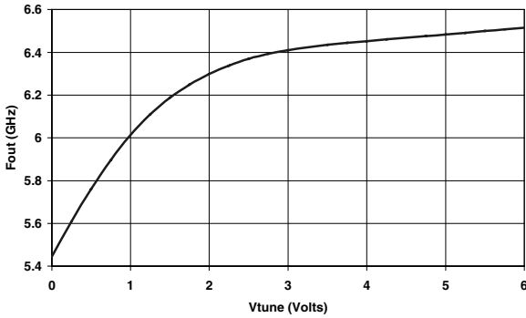
XQ1000-BD Output Frequency vs. Tuning Voltage
