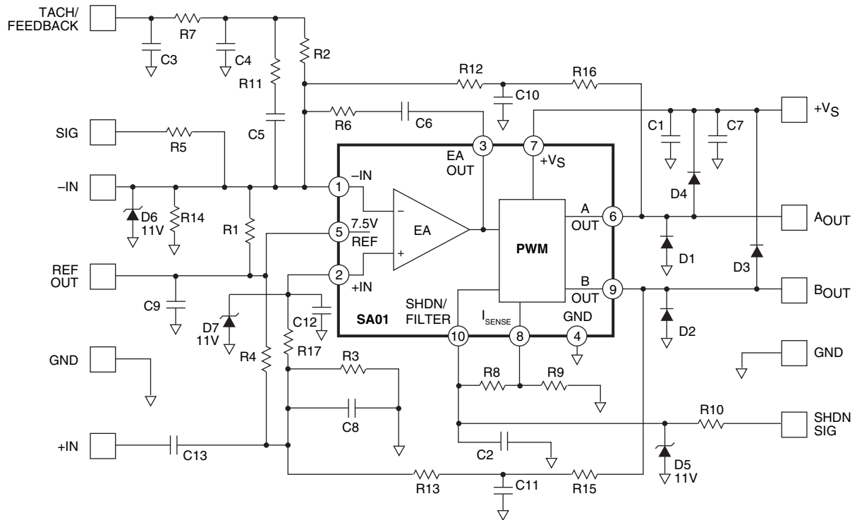
FIGURE 2. PCB SCHEMATIC.
