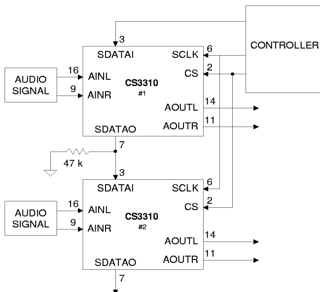
Figure 4. Daisy Chaining Diagram
