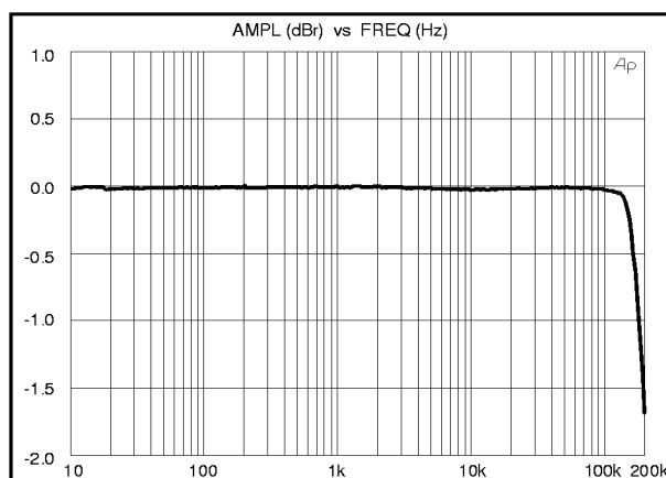
Figure 8. Frequency Response Full Scale Input
