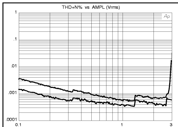
Figure 6. THD+N vs. AMP
