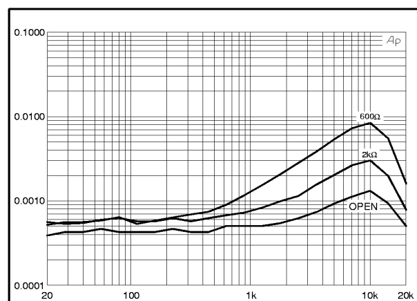
Figure 10. THD+N vs. Frequency LOAD = 600 \Omega , 2 k \Omega , open ckt
