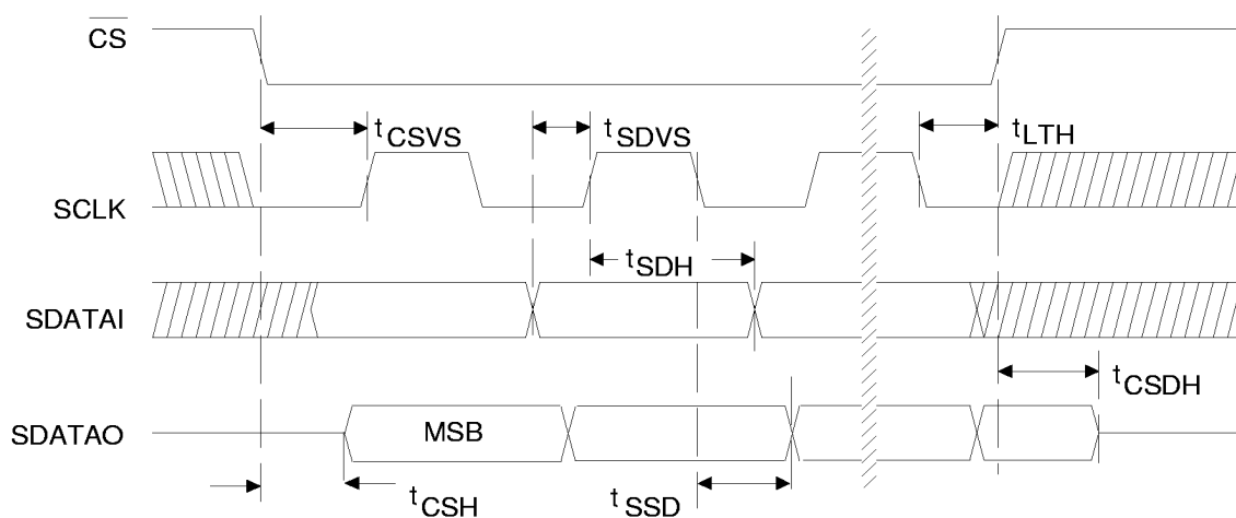
Figure 1. Serial Port Timing Diagram
