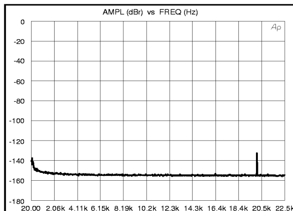
Figure 7. 20 kHz Crosstalk
