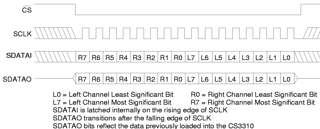
Figure 3. Serial Port Timing
