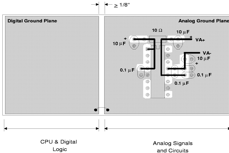
Figure 5. Recommended 2-Layer PCB Layout
