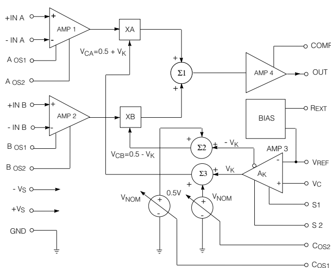
Fig. 1 Functional Block Diagram of the GT4122
