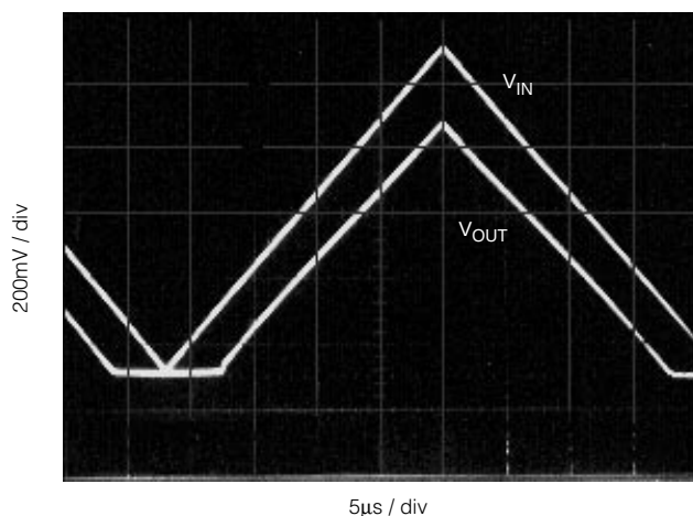
Photograph 4. CONTROL OFFSET (RV2) - fully c.c.w.
