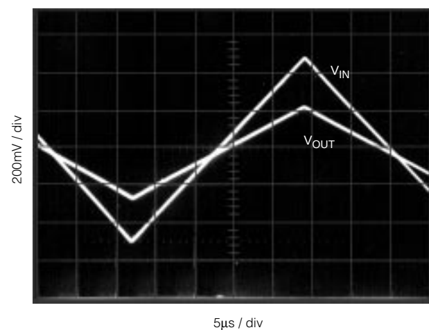
Photograph 5. 50% GAIN (RV1) - fully c.c.w. (min)
