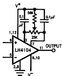
FIGURE 3. Offset Null*
