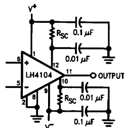
FIGURE 4. Using Resistor Current Limiting*
