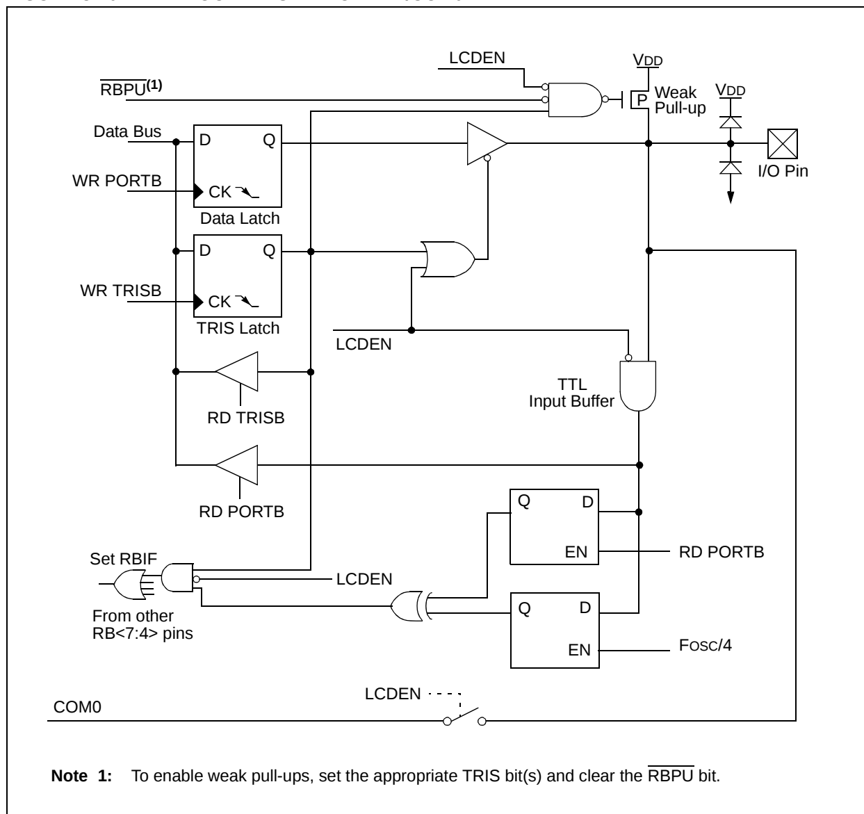
FIGURE 3-10: BLOCK DIAGRAM OF RB4/COM0
