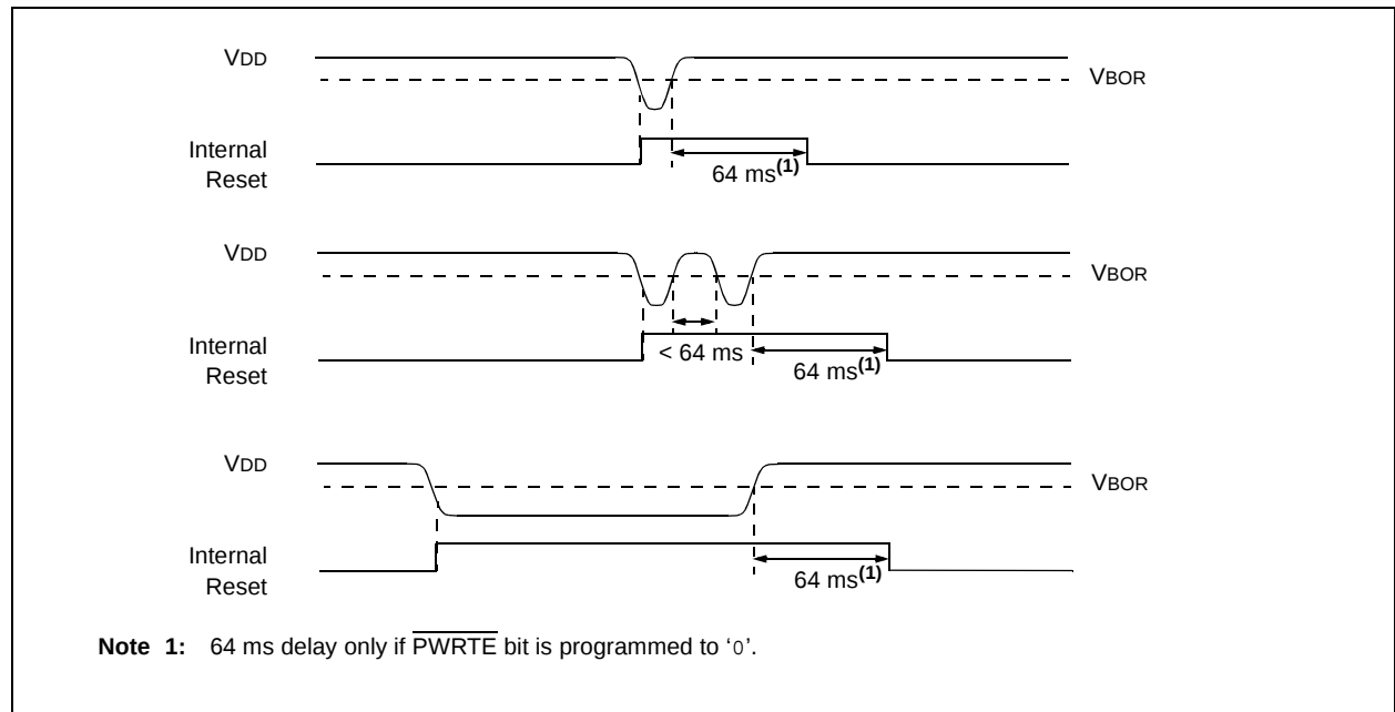
FIGURE 16-3: BROWN-OUT SITUATIONS
