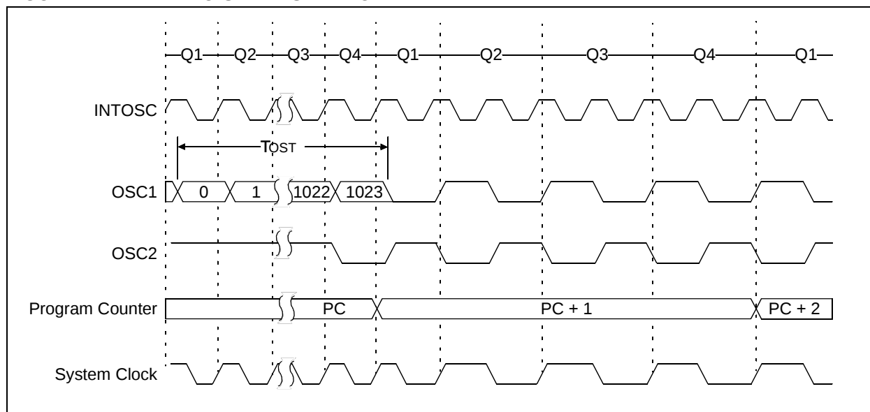
FIGURE 4-7: TWO-SPEED START-UP
