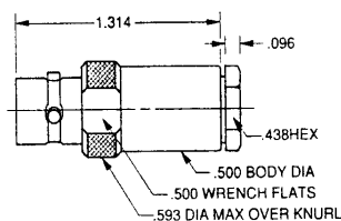
3-lug CJ70- ⚠ 2-lug CJ70TL- ⚠ 4-lug CJ70FL- ⚠ Threaded CJ370- ⚠
