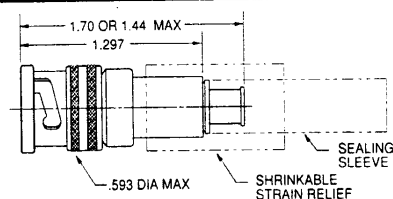
2-lug PL74C- ⚠ 3-lug PL75C- ⚠ 4-lug PL75CFL- ⚠ Threaded PL375C- ⚠
