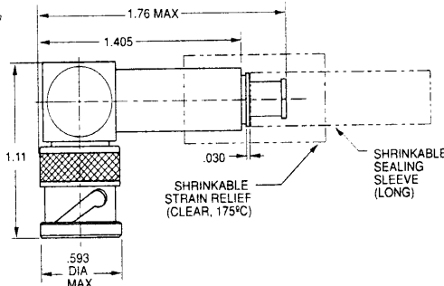
RIGHT ANGLE CABLE PLUG TOOL CRIMP
