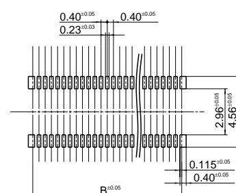
Recommended PC board pattern (TOP VIEW)
