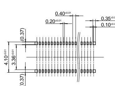
Recommended metal mask pattern Metal mask thickness: Here, 120 μm (Opening area ratio: 40%)
