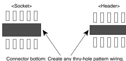
Connector bottom: Create any thru-hole pattern wiring.
