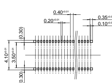
Recommended metal mask pattern Metal mask thickness: Here, 150 μm (Opening area ratio: 32%)
