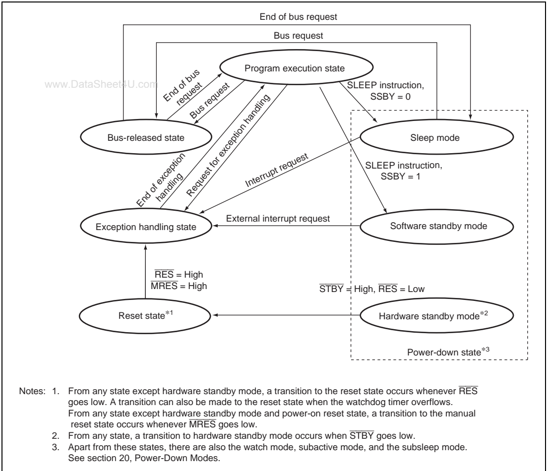
Figure 2.13 State Transitions
