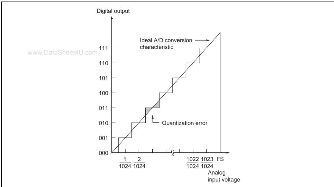
Figure 15.7 A/D Conversion Precision Definitions (1)
