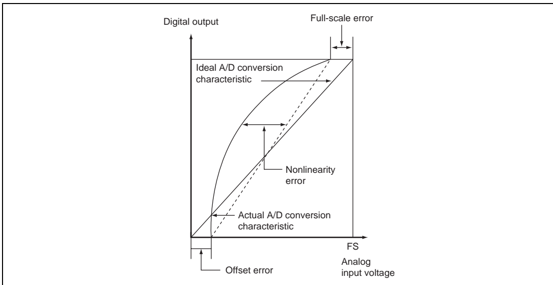
Figure 15.8 A/D Conversion Precision Definitions (2)
