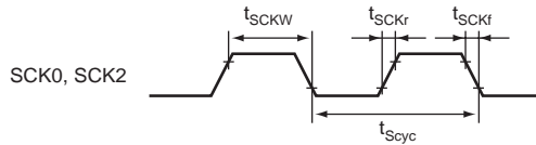
Figure 22.15 SCK Clock Input Timing
