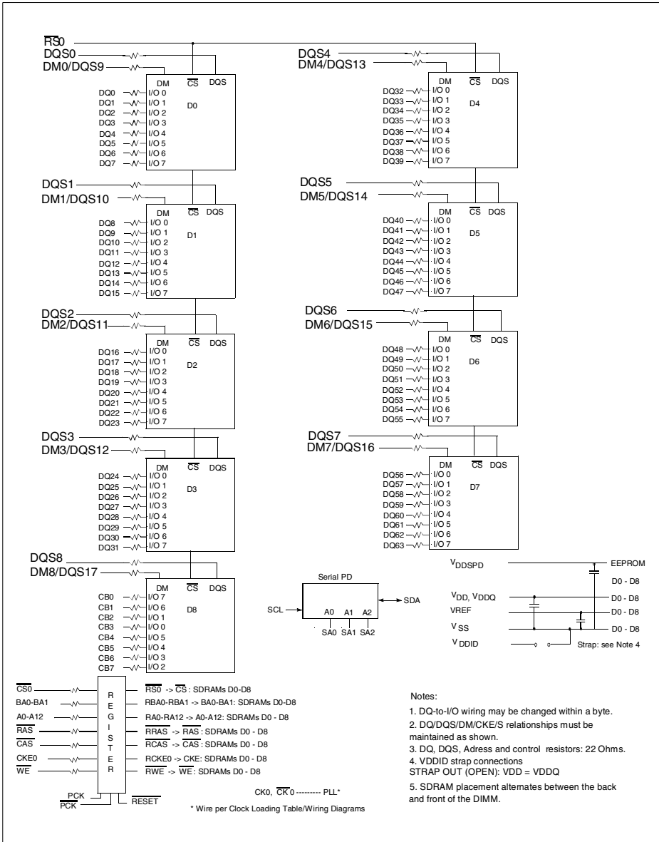
Block Diagram: One Bank 16Mb x 72 DDR-I SDRAM DIMM Module HYS72D16000GR using x8 organized SDRAMs on Raw Card Version A
