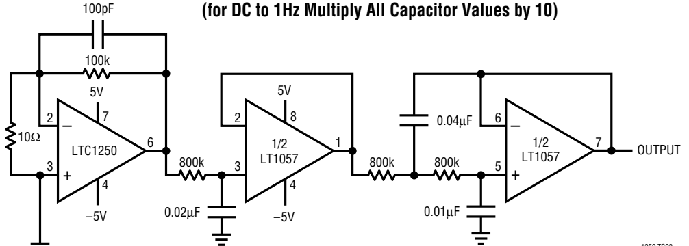
DC to 10Hz Noise Test Circuit (for DC to 1Hz Multiply All Capacitor Values by 10)
