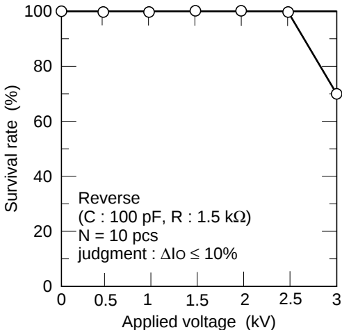
Electrostatic Destruction (Reverse)
