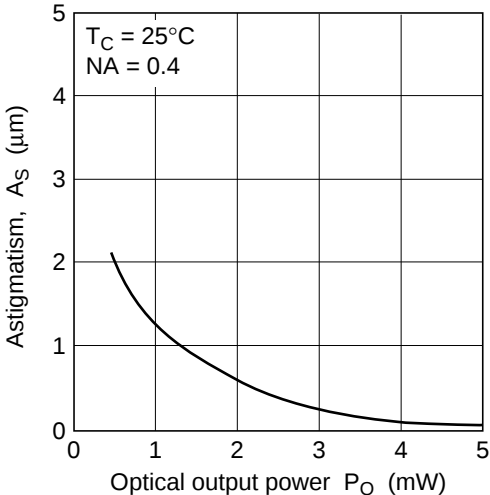
Astigmatism vs. Optical Output Power
