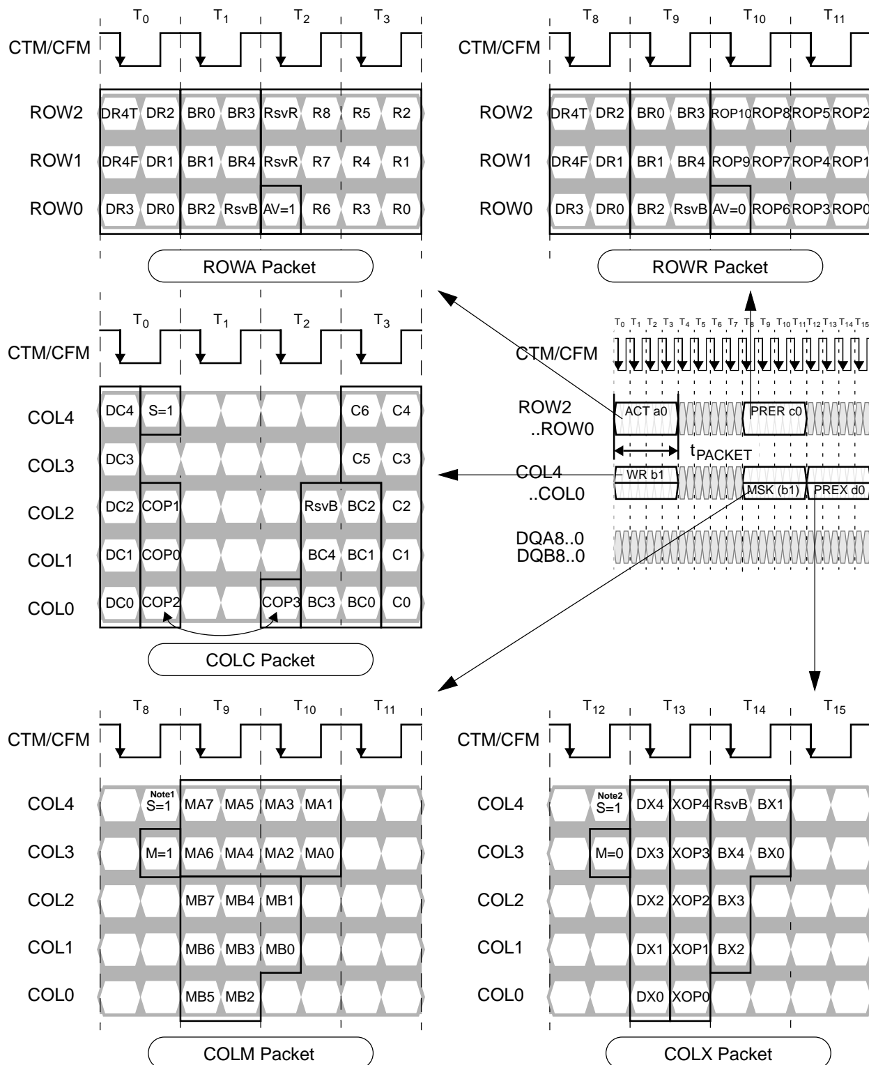
Figure 2-1 Packet Formats
