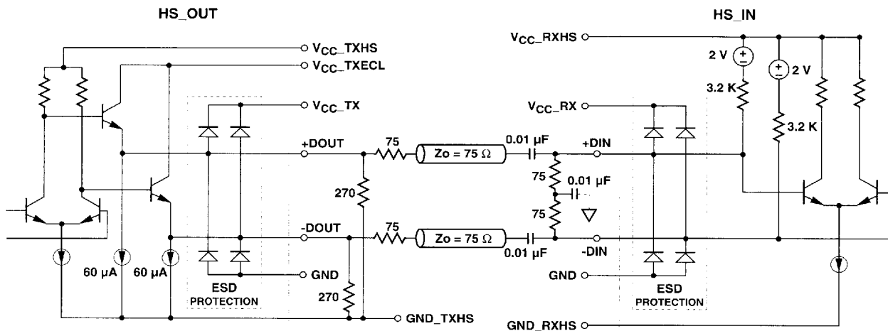
Figure 10. HS_OUT and HS_IN Simplified Circuit Schematic.
