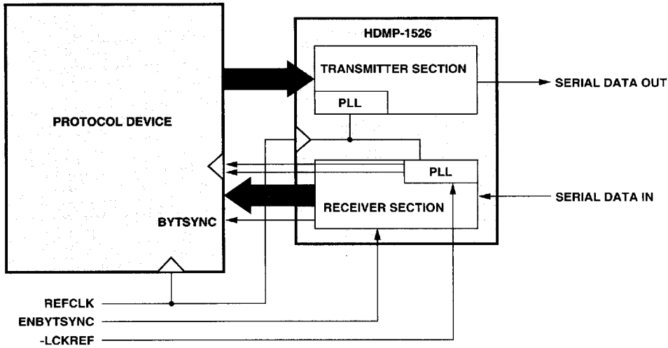
Figure 1. Typical Application Using the HDMP-1526.
