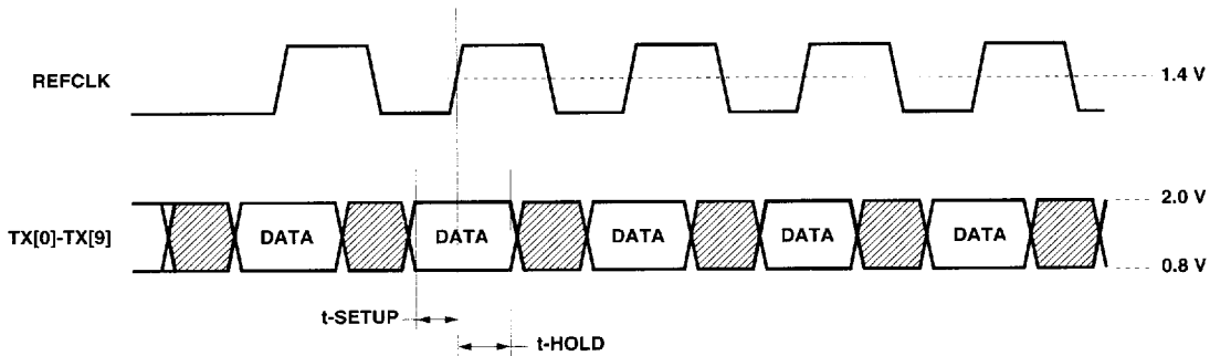
Figure 3. Transmitter Section Timing.
