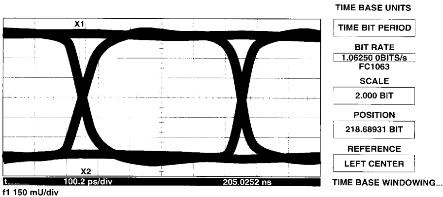
b. Single-Ended HS_OUT Output (Dout+).
