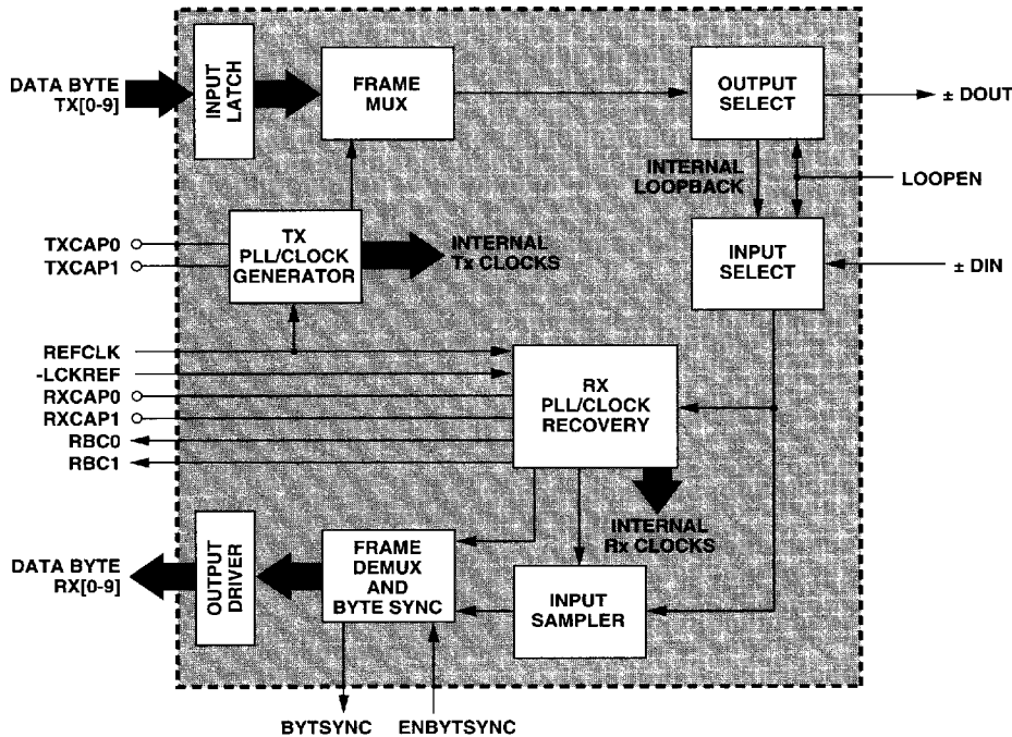
Figure 2. HDMP-1526 Transceiver Block Diagram.
