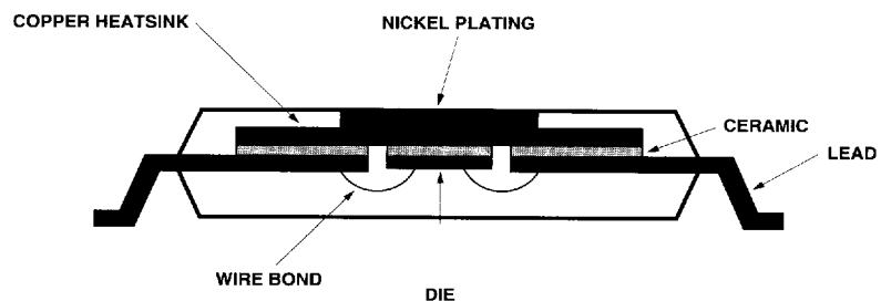
Figure 13. Package Cross Section of HDMP-1526.
