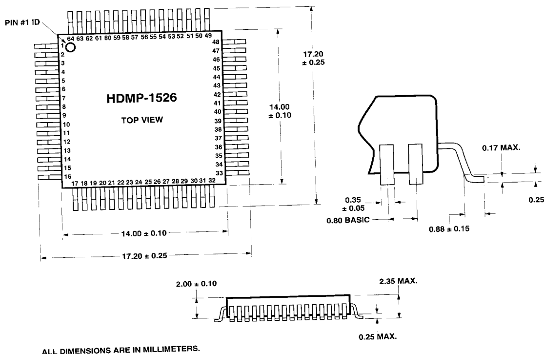
Figure 14. Mechanical Dimensions of HDMP-1526.
