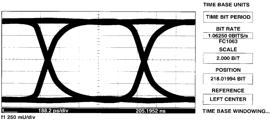
a. Differential HS_OUT Output (Dout+ Minus Dout-).
