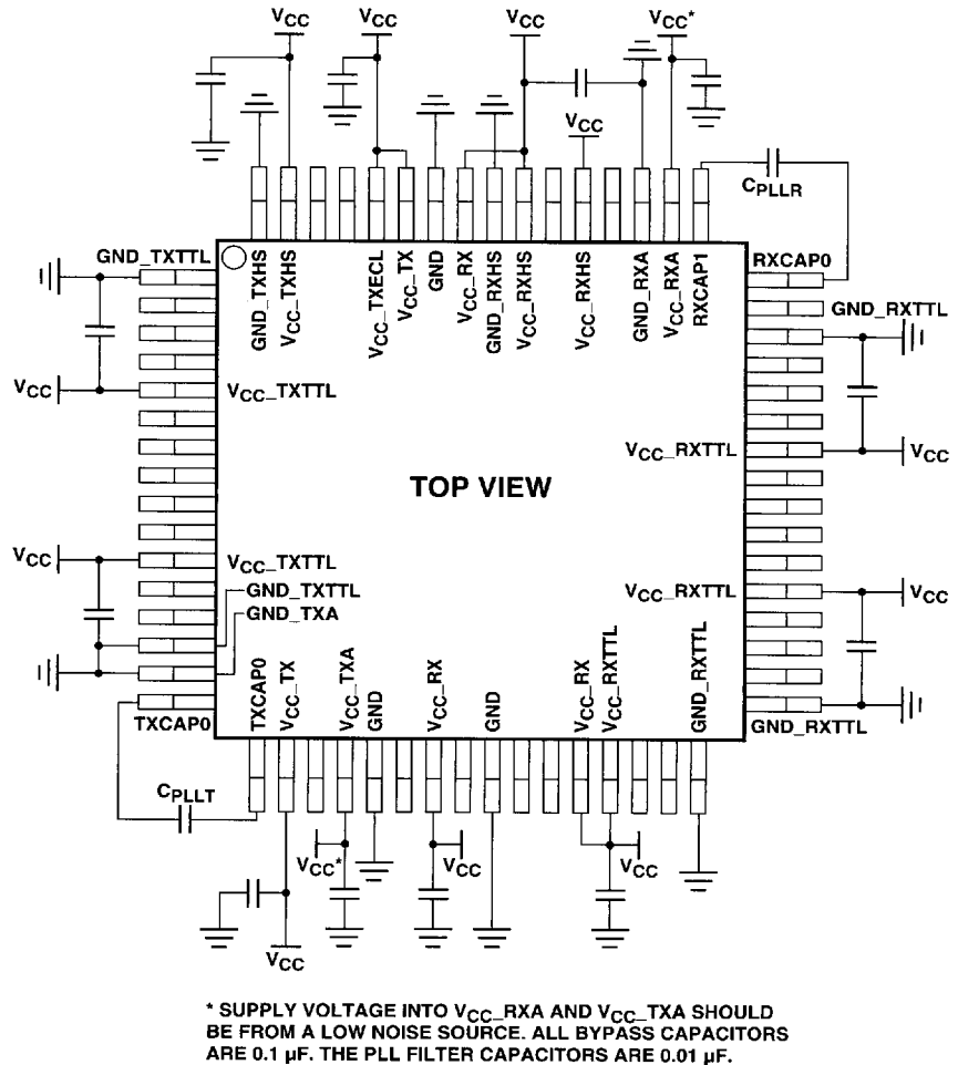
Figure 12. Power Supply Bypass.
