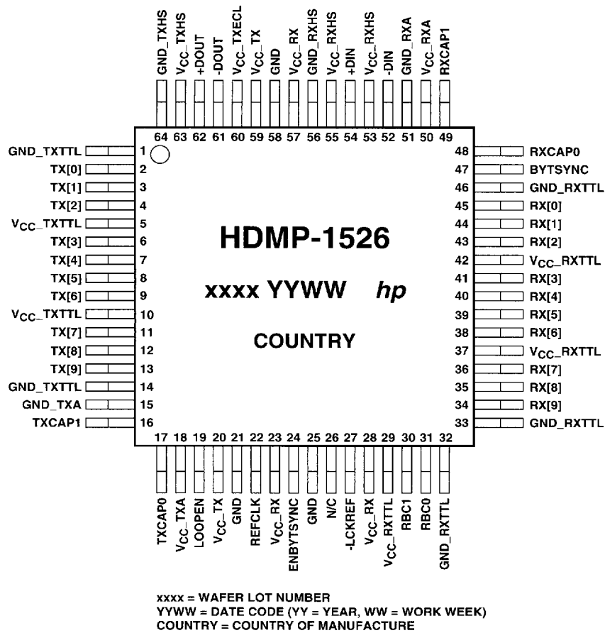
Figure 11. HDMP-1526 (TRx) Package Layout and Marking, Top View.
