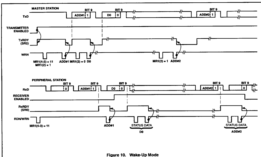
Figure 10. Wake-Up Mode
