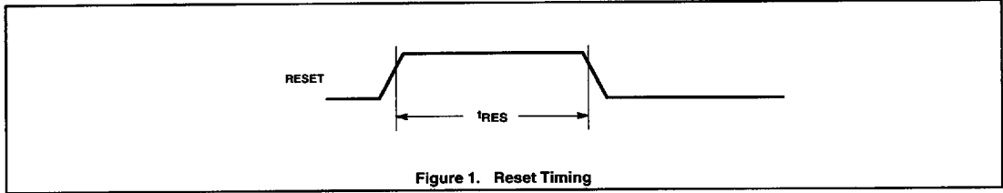
Figure 1. Reset Timing
