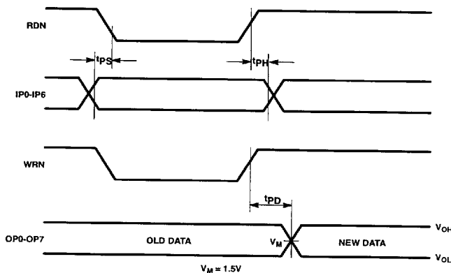
Figure 3. Port Timing
