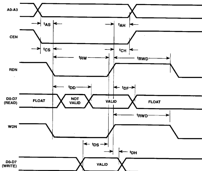
Figure 2. Bus Timing
