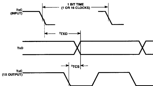
Figure 6. Transmit
