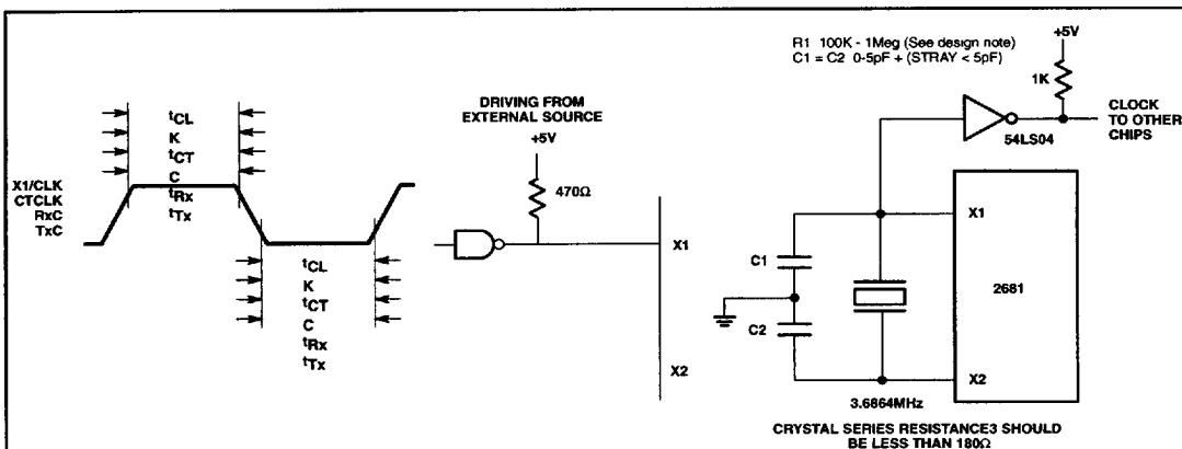
Figure 5. Clock Timing
