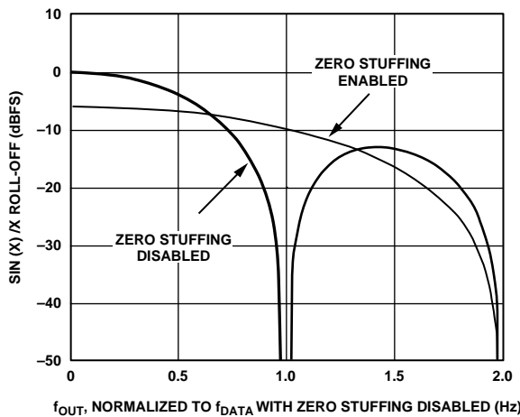
Figure 75. Effect of Zero Stuffing on DAC's \text{SIN}(x)/x Response
