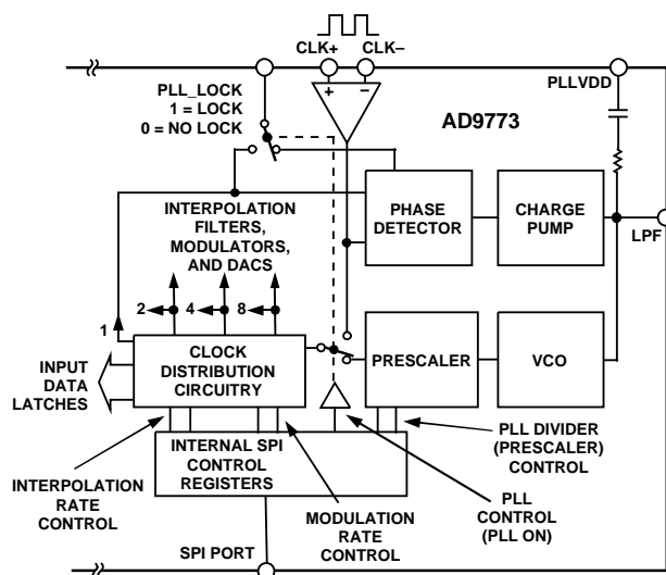
Figure 45. PLL and Clock Circuitry with PLL Enabled
