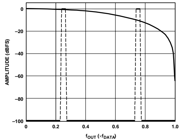
Figure 61. No Interpolation, Modulation = f_{DAC}/4
