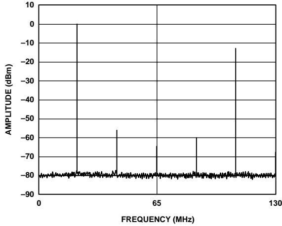
Figure 6. Single-Tone Spectrum @ f_{DATA} = 65 MSPS with f_{OUT} = f_{DATA}/3
