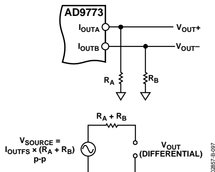
Figure 97. DAC Output Equivalent Circuit
