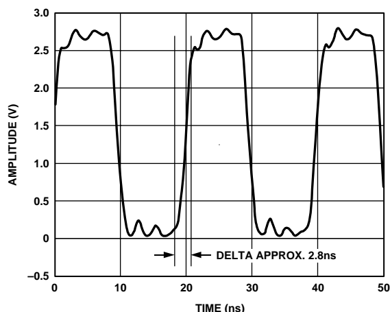
Figure 53. DATACLK Driver Capability into 330 Ω at 50 MHz
