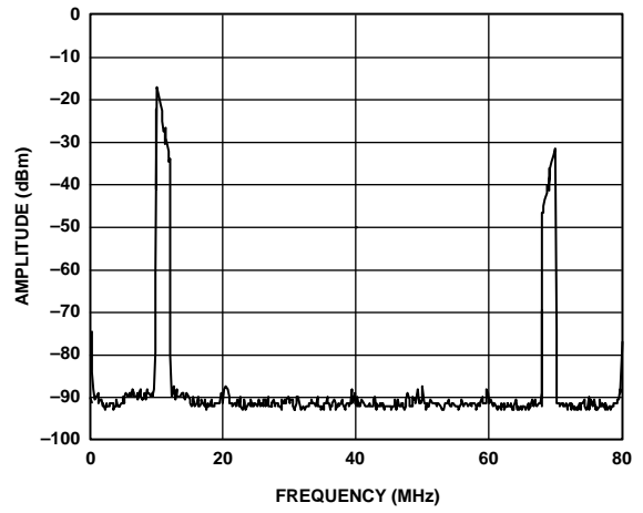
Figure 95. AD9773 Real DAC Output of Complex Input Signal Near Baseband (Positive Frequencies Only), Interpolation = 8x, Complex Modulation in AD9773 = +f_{DAC}/8
