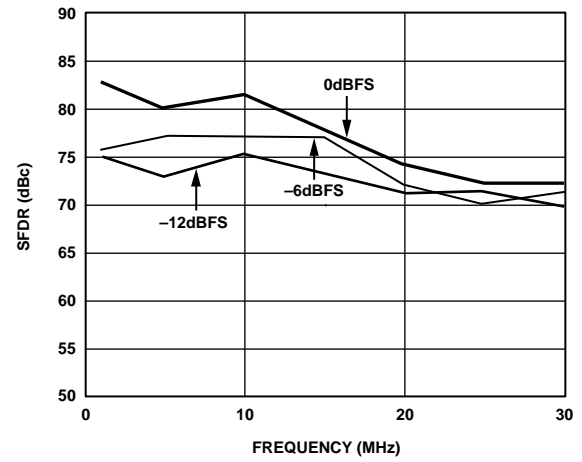
Figure 10. In-Band SFDR vs. f_{OUT} @ f_{DATA} = 78 MSPS
