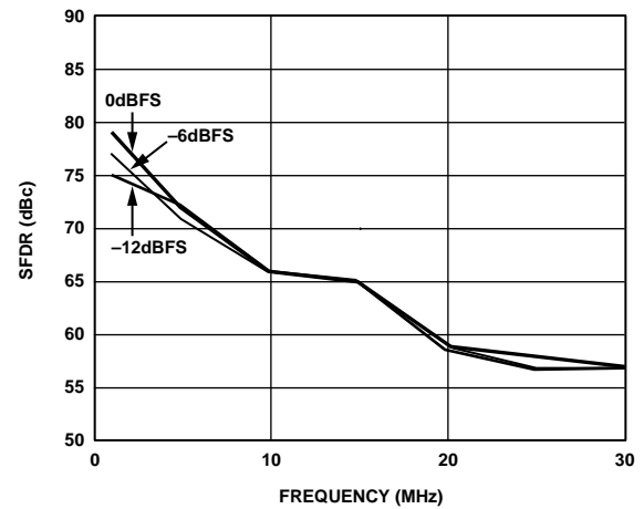
Figure 11. Out-of-Band SFDR vs. f_{OUT} @ f_{DATA} = 78 MSPS
