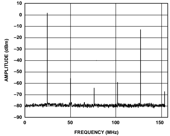
Figure 9. Single-Tone Spectrum @ f_{DATA} = 78 MSPS with f_{OUT} = f_{DATA}/3
