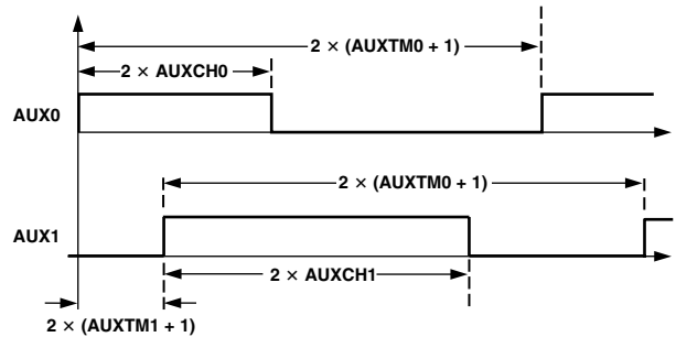
Figure 18b. Typical Auxiliary PWM Signals (All Times in Increments of t_{\text{CK}} ), Offset Mode
