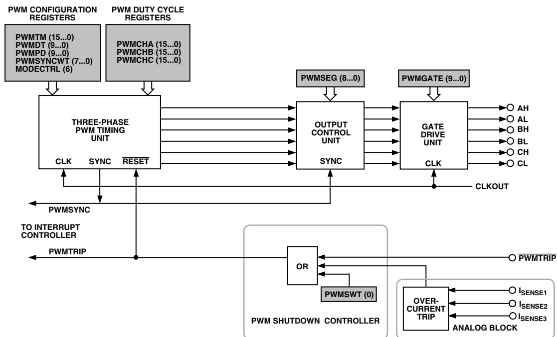
Figure 6. Overview of the PWM Controller of the ADC(F)341
