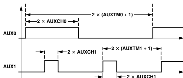
Figure 18a. Typical Auxiliary PWM Signals (All Times in Increments of t_{\text{CK}} ), Independent Mode
