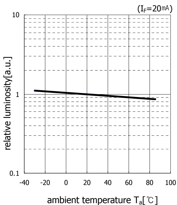
(4) ambient temperature vs. relative luminosity
