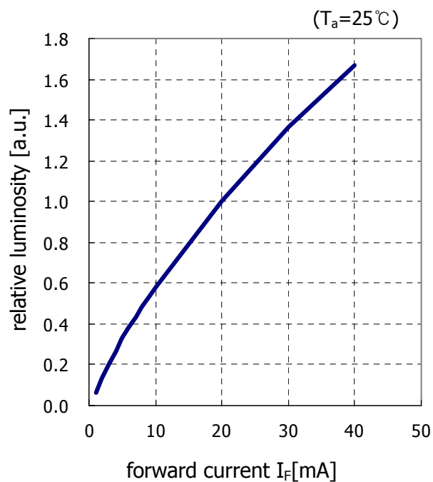
(2) forward current vs. relative luminosity
