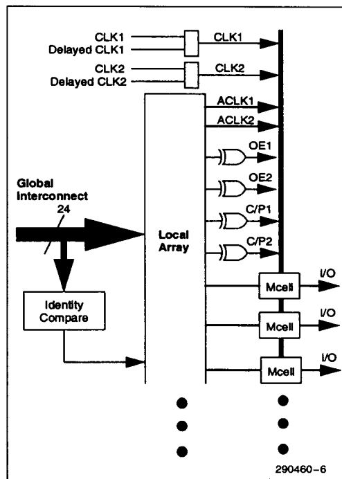
Figure 4. Control Signals
