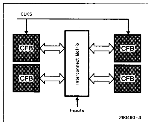
Figure 1. Interconnect Matrix
