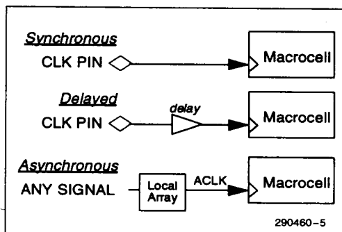
Figure 3. Clock Modes
