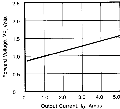
Diode Forward Voltage vs Output Current
