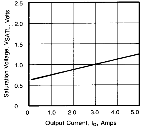
Sink Saturation Voltage vs Output Current
