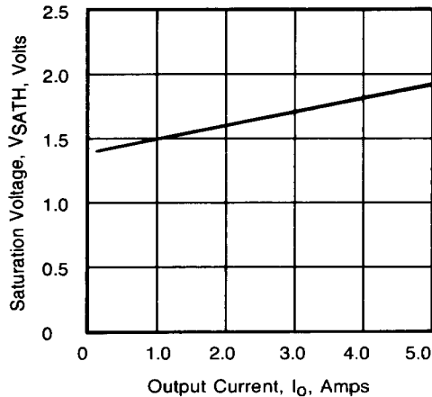
Source Saturation Voltage vs Output Current
