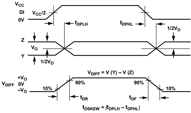
Figure 9. Driver Propagation Delays
