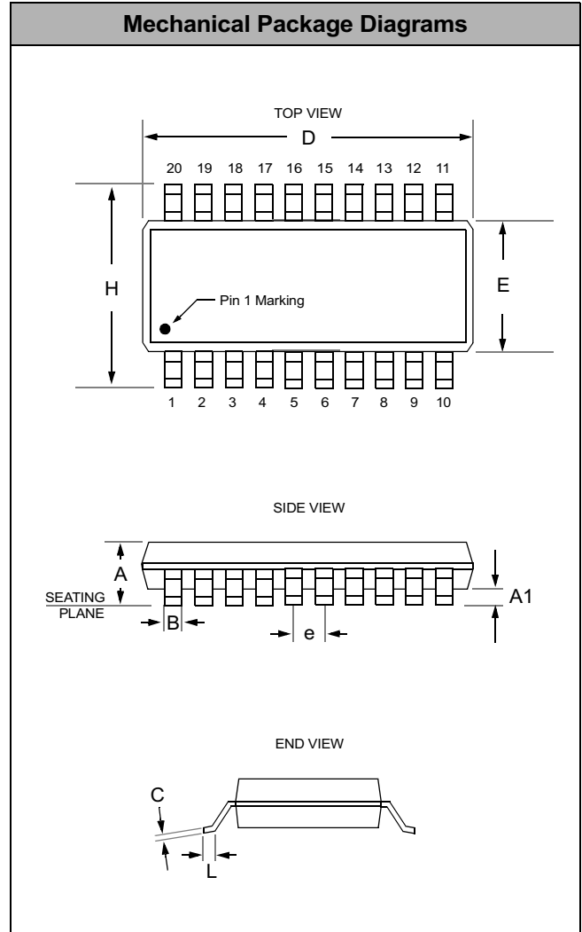
Package Dimensions for TSSOP-20
