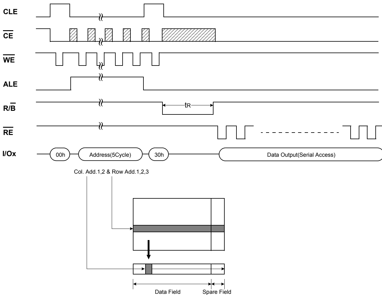
[Figure 8] Read Operation
