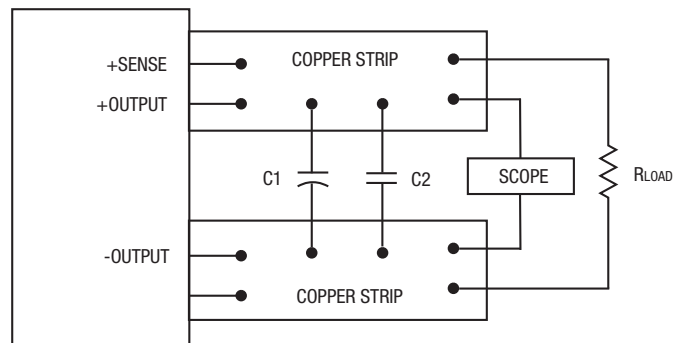
C1 = 0.1µF CERAMIC C2 = 10µF TANTALUM LOAD 2-3 INCHES (51-76mm) FROM MODULE Figure 3: Measuring Output Ripple and Noise (PARD)
