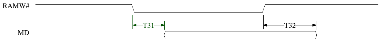
Figure 3.11 CPU Write DRAM Cycle
